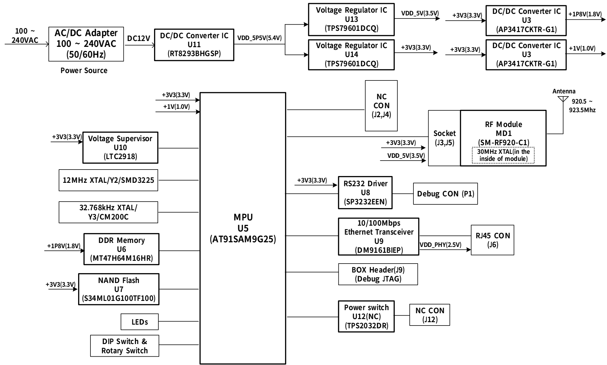
TGBS900BA(Base Station) Board Block Diagram
