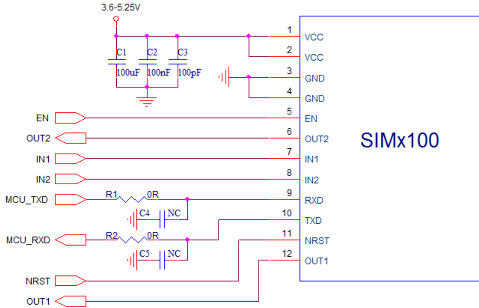
Simplified Reference Circuit
