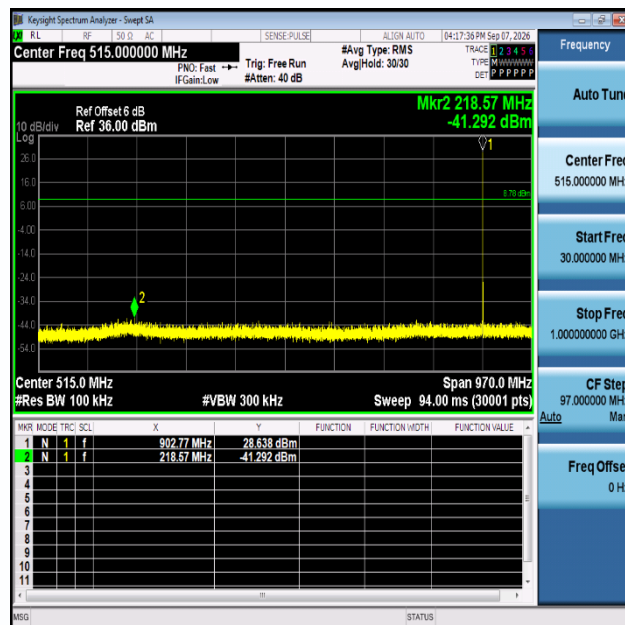
900M-Ant1-902.75-30~1000-PASS
