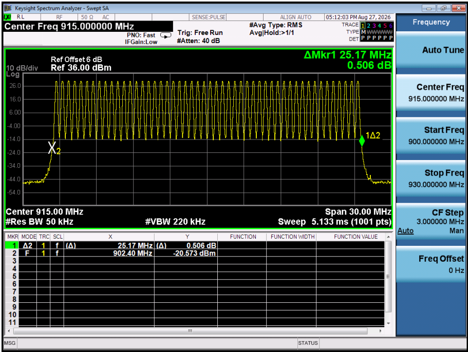
Hopping
