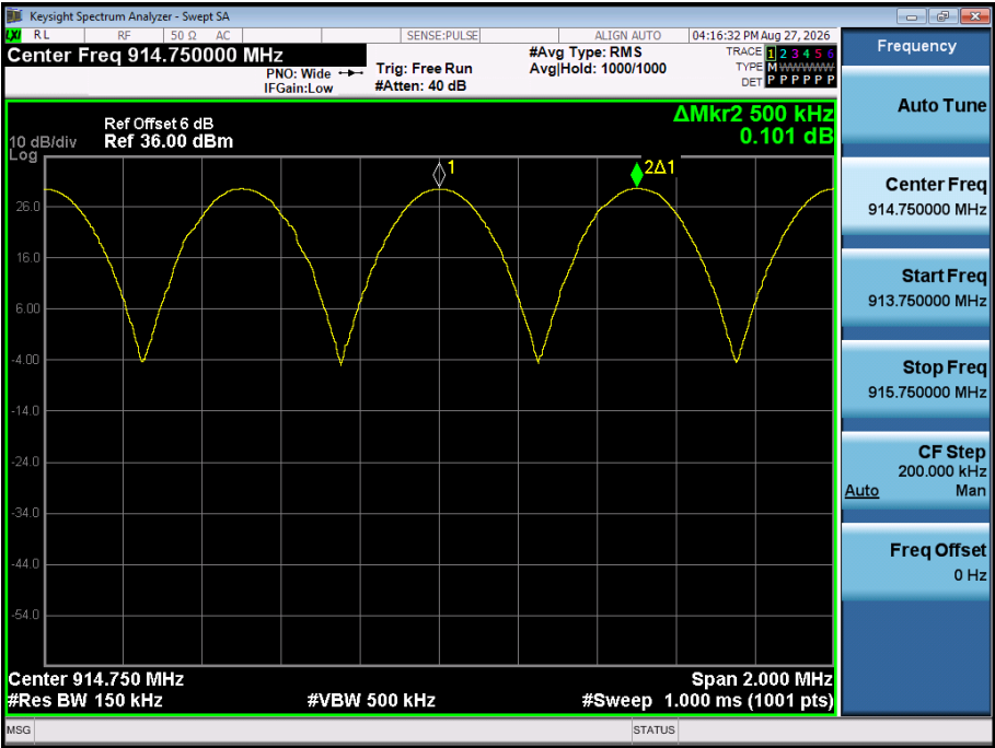
Hopping
