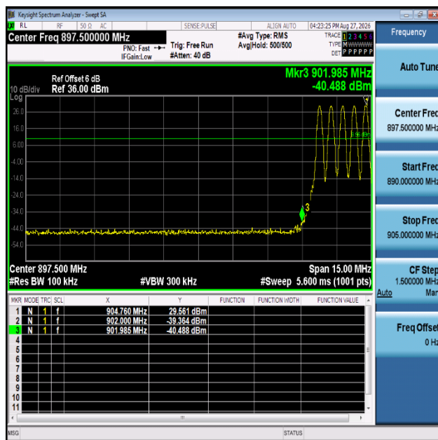
For Low channel Hopping Mode
