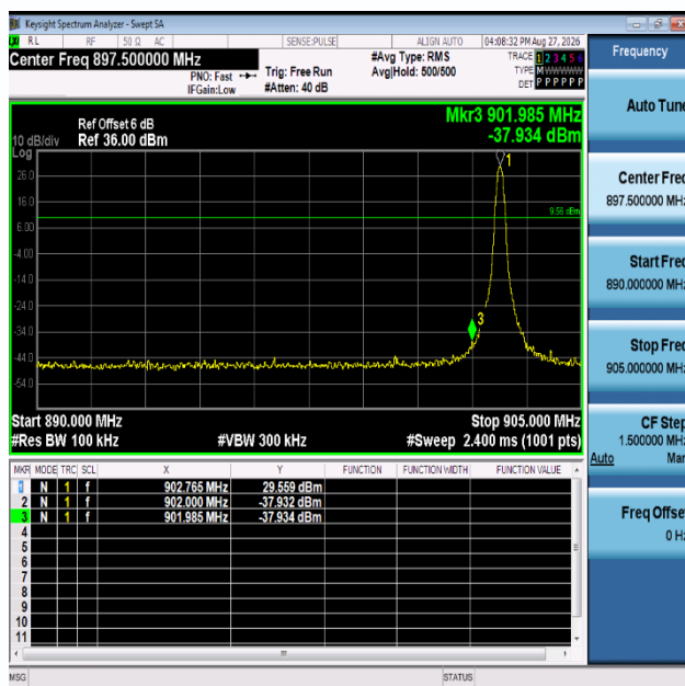
For Low channel Non-Hopping Mode
