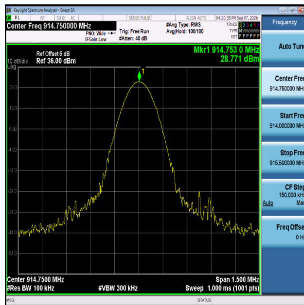
900M-Ant1-914.750~Reference-PASS
