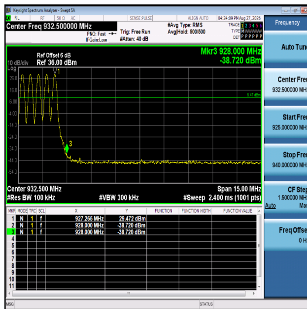
For High channel Hopping Mode
