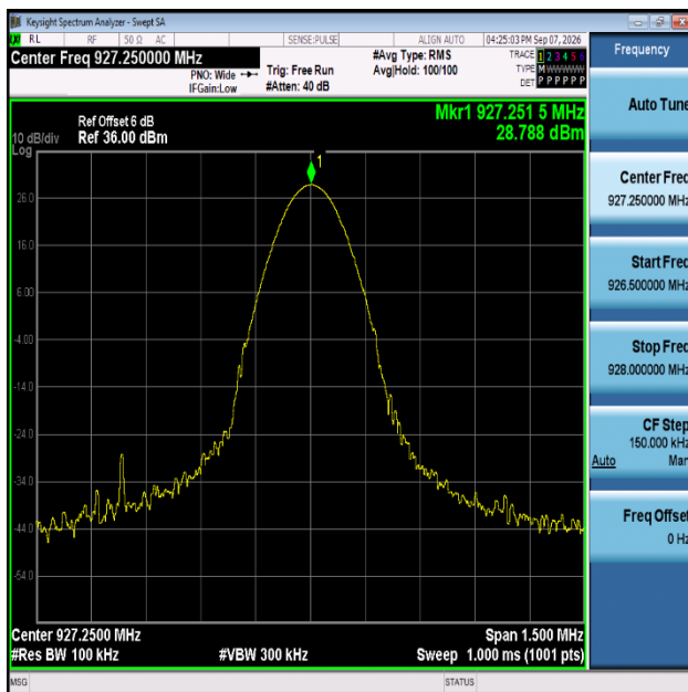
900M-Ant1-927.25-0~Reference-PASS
