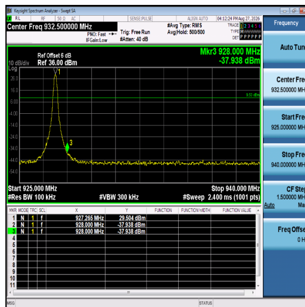
For High channel Non-Hopping Mode
