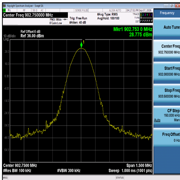
900M-Ant1-902.750~Reference-PASS
