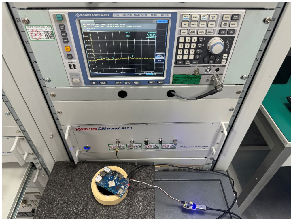
RF CONDUCTION Measurement Photo
