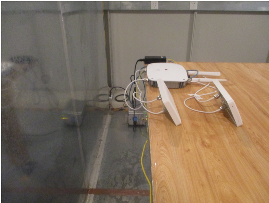
AC power line conducted emissions Side View
