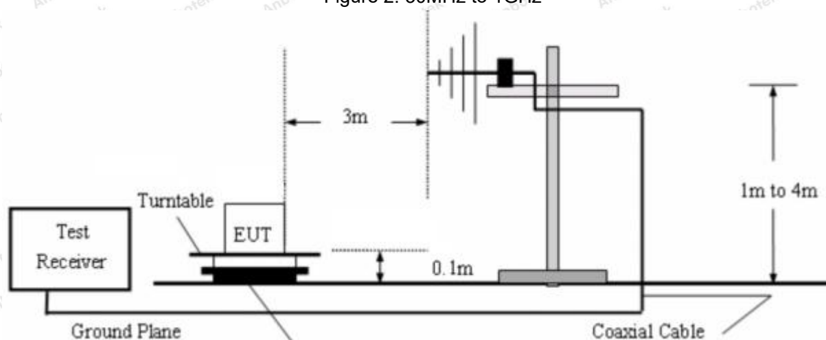
Figure 3. Above 1 GHz
