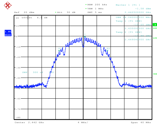
b_2442MHz_Chain 0 14.040MHz
