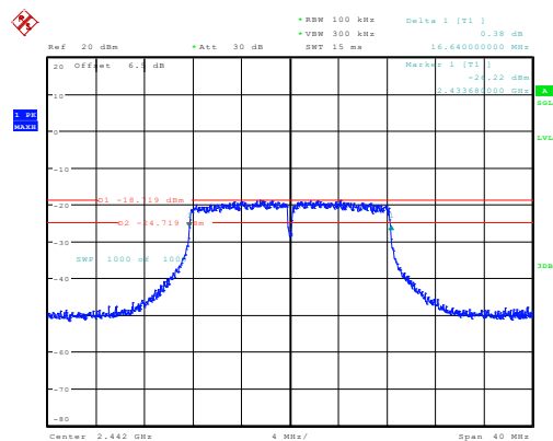
g_2442MHz_Chain 0 16.640MHz
