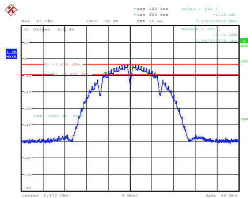
b_2472MHz_Chain 0 9.160MHz
