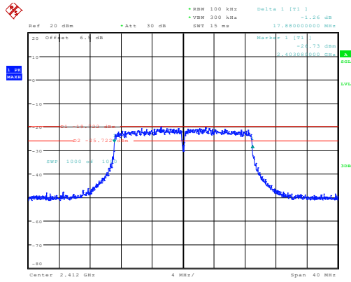
n20_2412MHz_Chain 0 17.880MHz
