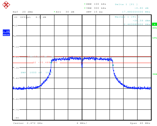
n20_2472MHz_Chain 0 17.880MHz
