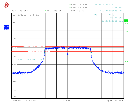
g_2412MHz_Chain 0 16.640MHz
