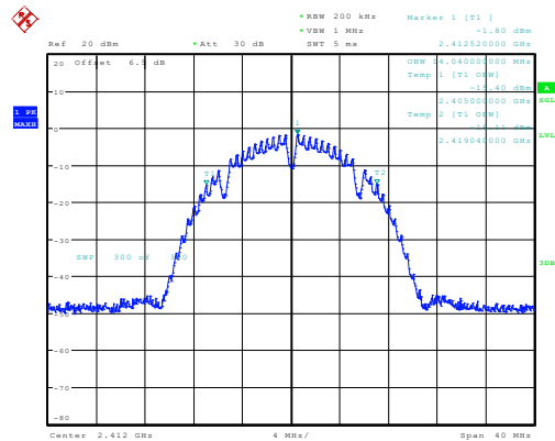
b_2412MHz_Chain 0 14.040MHz
