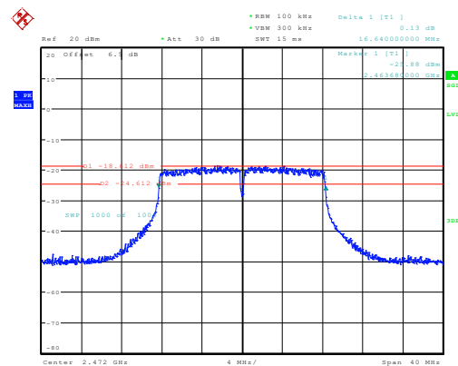
g_2472MHz_Chain 0 16.640MHz
