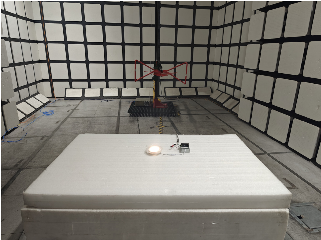
Radiated Emissions View (Below 1 GHz) (Model: H601E)
