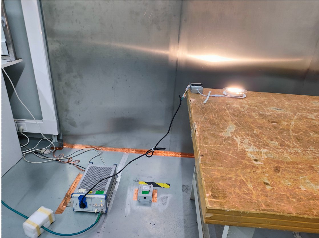
Conducted Emissions - Side View(Model: H601E)
