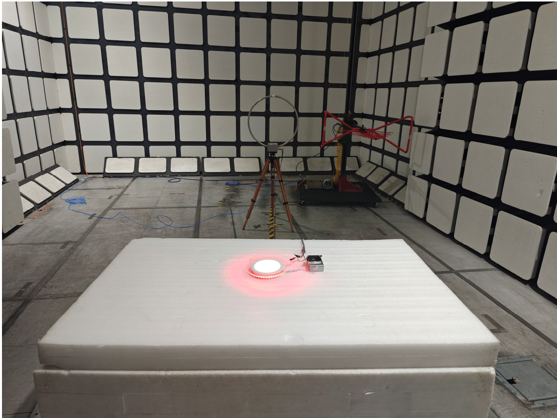
Radiated Emissions View (Below 1 GHz) (Model: H601F)
