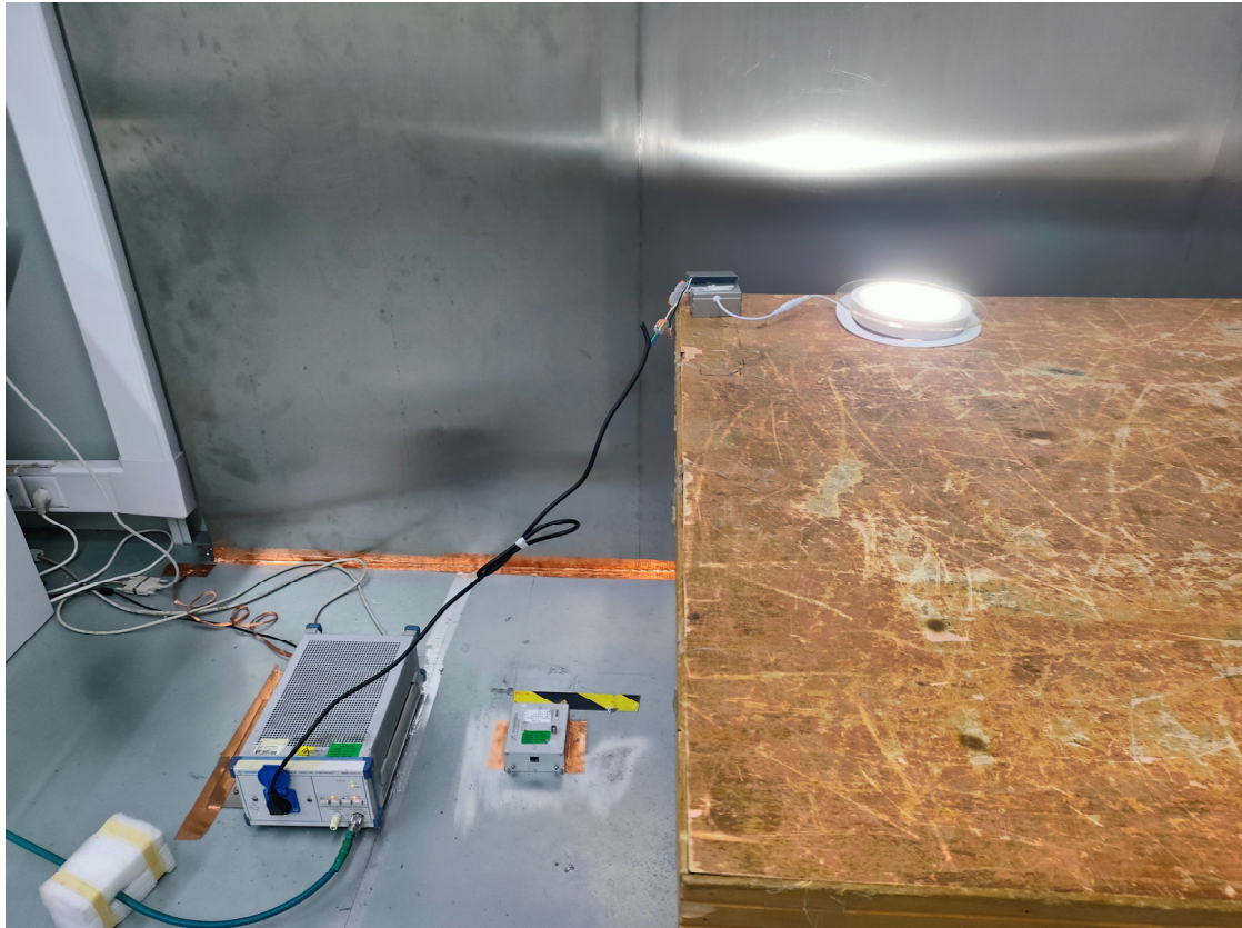
Conducted Emissions - Side View(Model: H601F)
