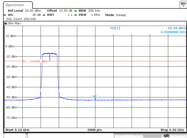
802.11a_5200MHz_Chain 1
