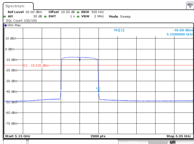
802.11ax40_5230MHz_RU_FULL_Chain 0
