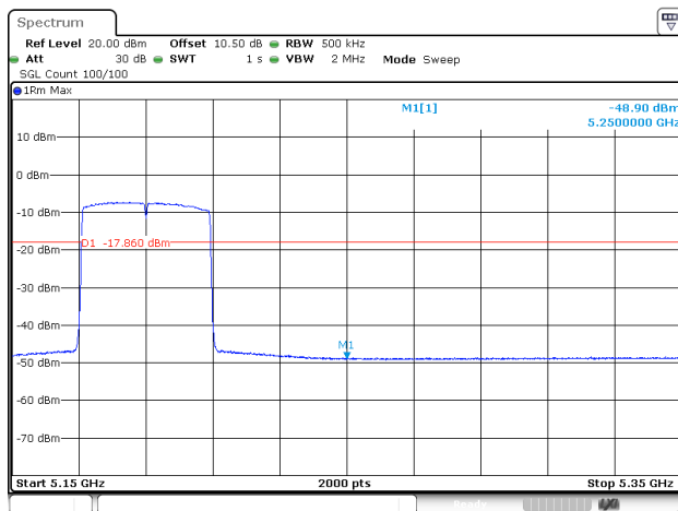
802.11ax40_5190MHz_RU_FULL_Chain 1
