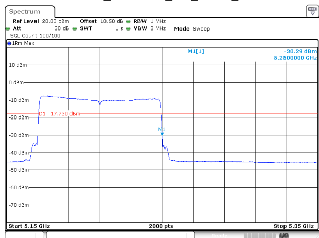
802.11ax80_5210MHz_RU_FULL_Chain 1
