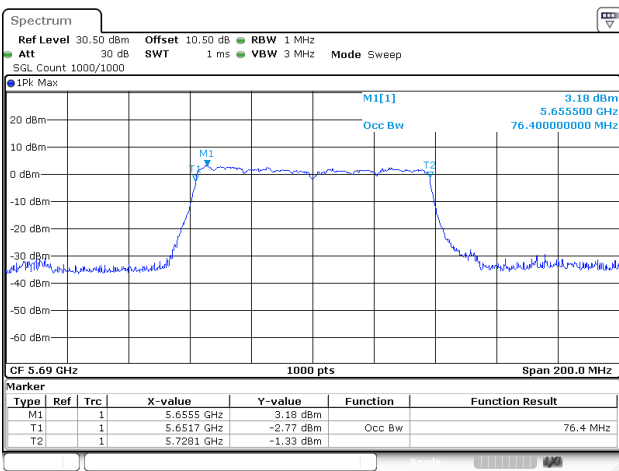
802.11ac80_5690MHz_Chain 0
