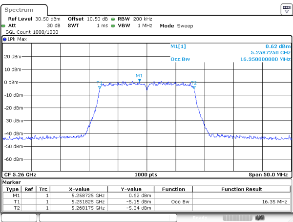
802.11a_5260MHz_Chain 1
