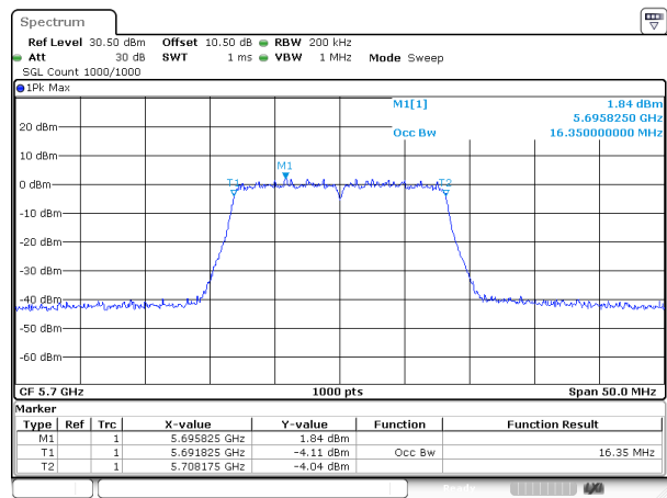
802.11a_5700MHz_Chain 0
