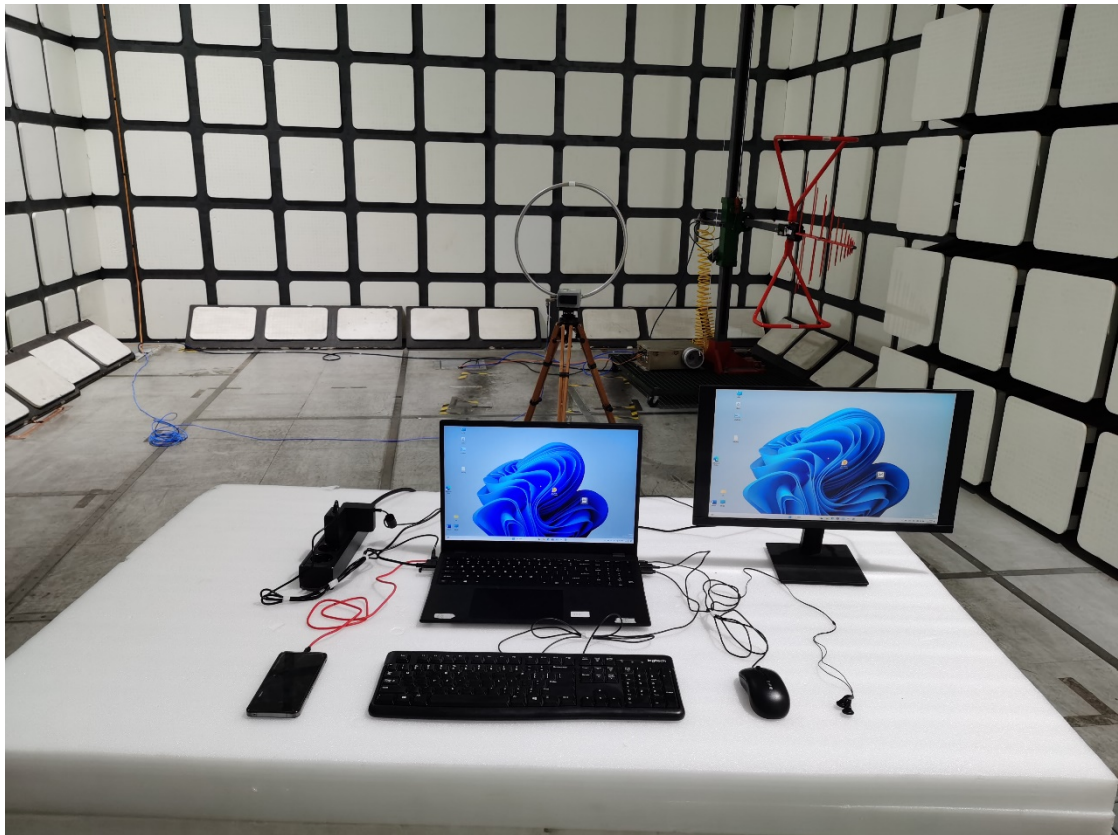
Radiated Emissions View (Below 30MHz) Adapter 3
