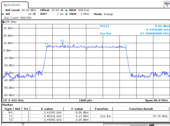
802.11ax40_2422MHz_RU_Full_Chain 0
