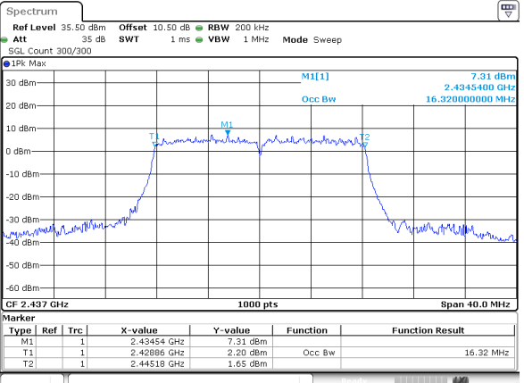
802.11g_2437MHz_Chain 0
