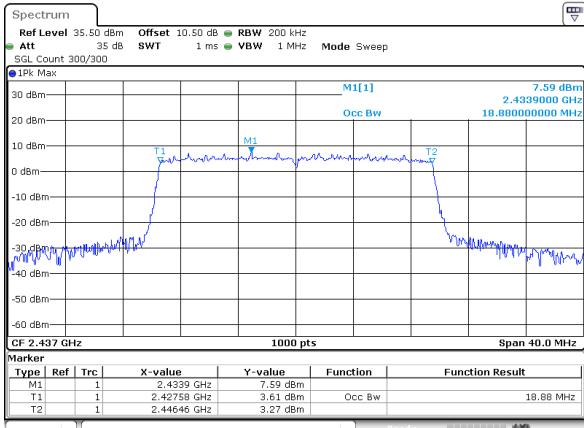
802.11ax20_2437MHz_RU_Full_Chain 1
