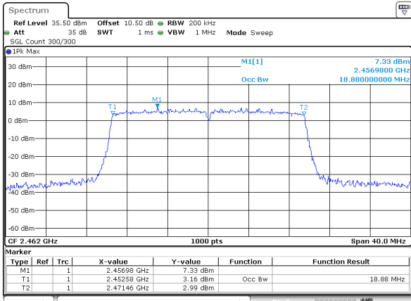
802.11ax20_2462MHz_RU_Full_Chain 0
