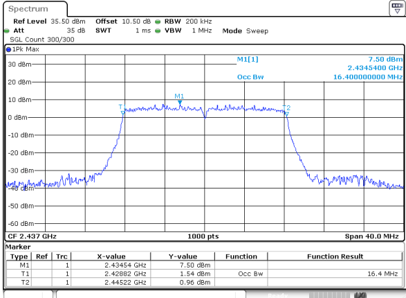
802.11g_2437MHz_Chain 1
