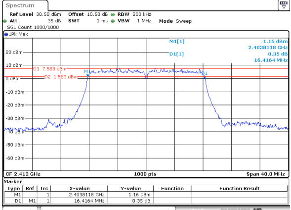
802.11g_2412MHz_Chain 1
