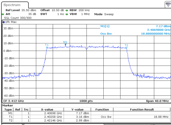
802.11ax20_2412MHz_RU_Full_Chain 0
