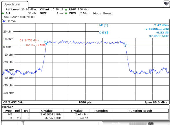
802.11ax40_2452MHz_RU_Full_Chain 0
