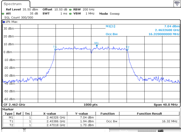
802.11g_2462MHz_Chain 0
