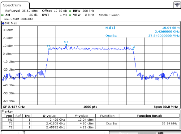
802.11ax40_2437MHz_RU_Full_Chain 0
