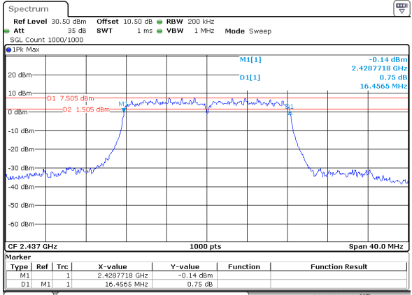
802.11g_2437MHz_Chain 0
