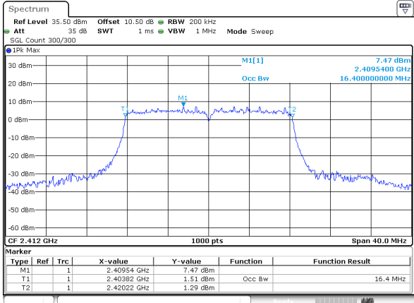
802.11g_2412MHz_Chain 0
