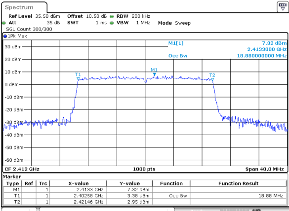
802.11ax20_2412MHz_RU_Full_Chain 1
