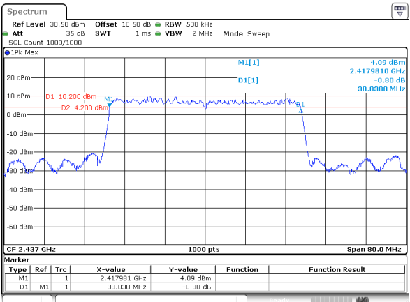
802.11ax40_2437MHz_RU_Full_Chain 0
