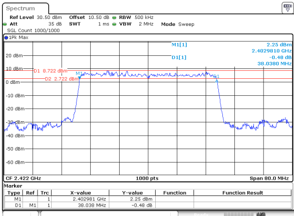
802.11ax40_2422MHz_RU_Full_Chain 0
