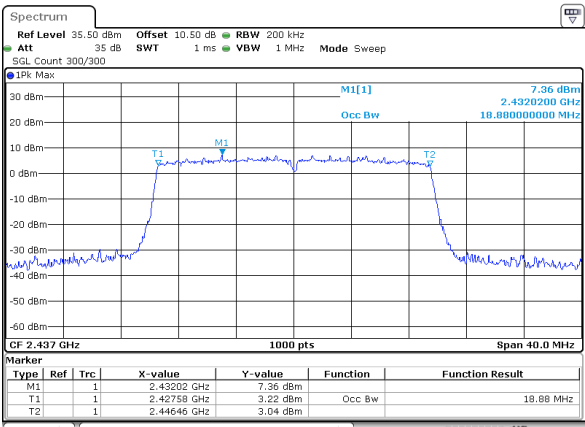
802.11ax20_2437MHz_RU_Full_Chain 0
