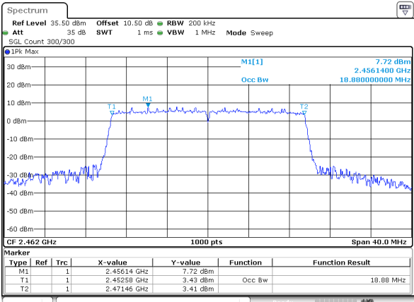
802.11ax20_2462MHz_RU_Full_Chain 1
