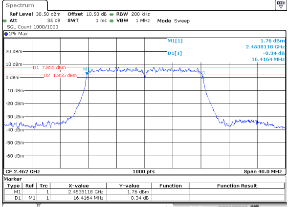
802.11g_2462MHz_Chain 1
