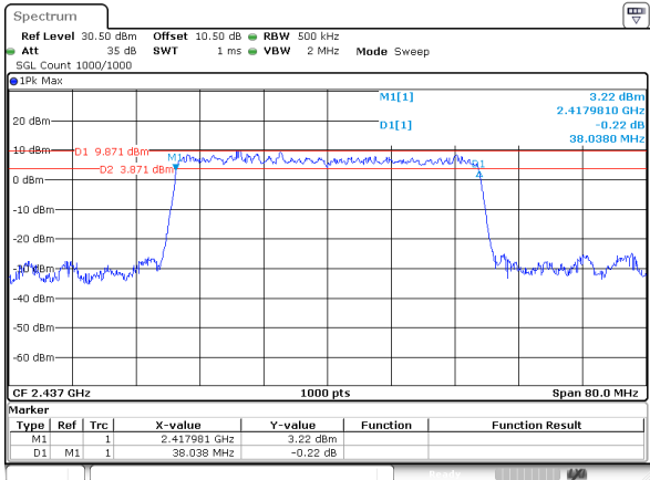
802.11ax40_2437MHz_RU_Full_Chain 1
