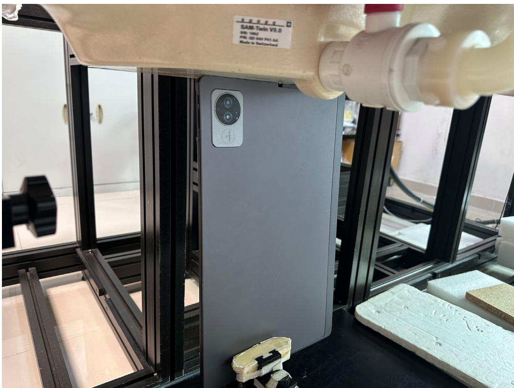
WWAN Body Left Setup Photo (0 mm)
