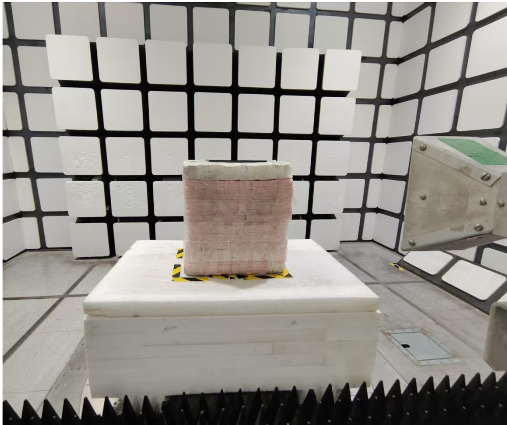
Radiated Emissions View (18-40 GHz)
