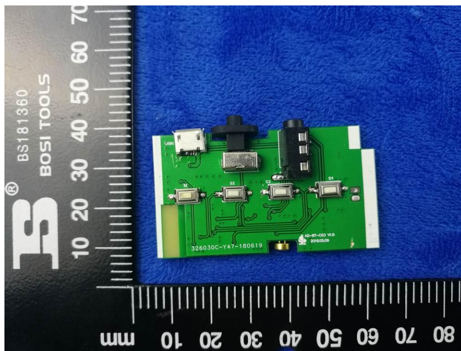
Mainboard-Rear View
