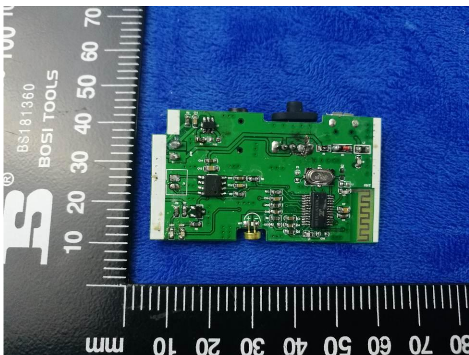
Mainboard-Front View
