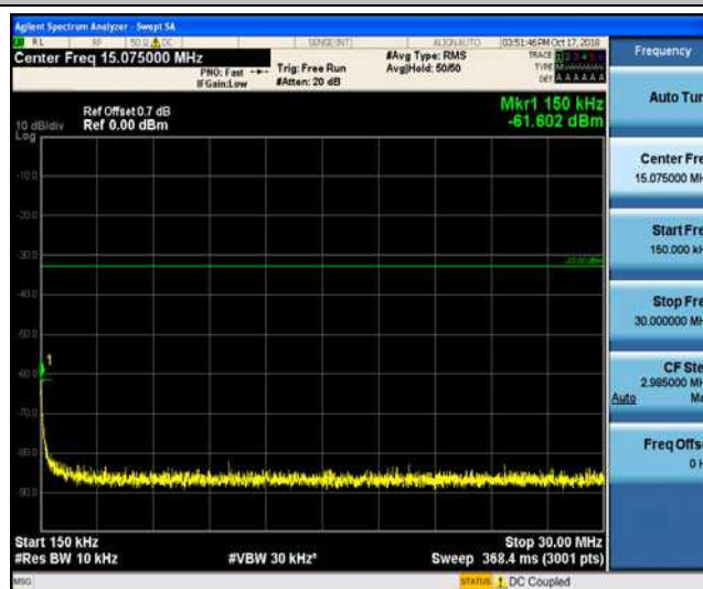
Band2_5MHz_16QAM_18625_1RB#0
