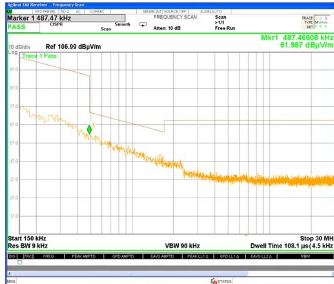
Plot # 27. Investigation result in 0.15 – 30 MHz frequency range.
