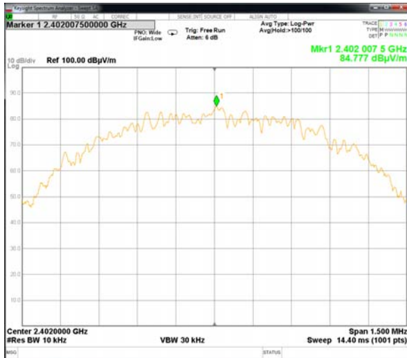
Plot # 7. Carrier frequency – 2402 MHz
