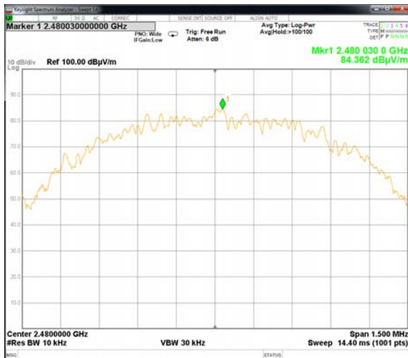
Plot # 9. Carrier frequency – 2480 MHz
