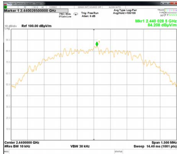
Plot # 8. Carrier frequency – 2440 MHz
