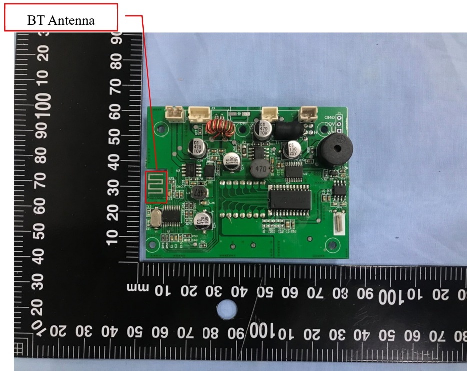
Antenna View
