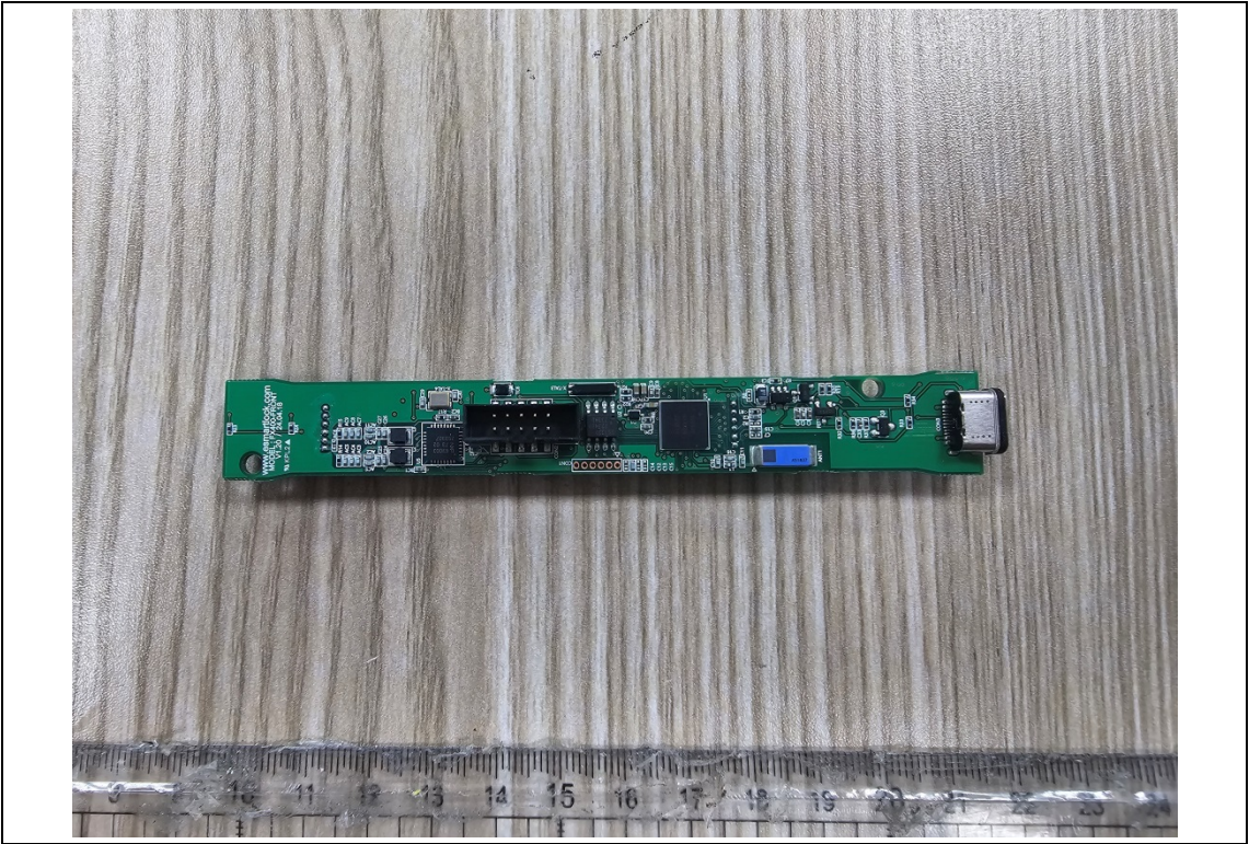
Board 3 Rear
