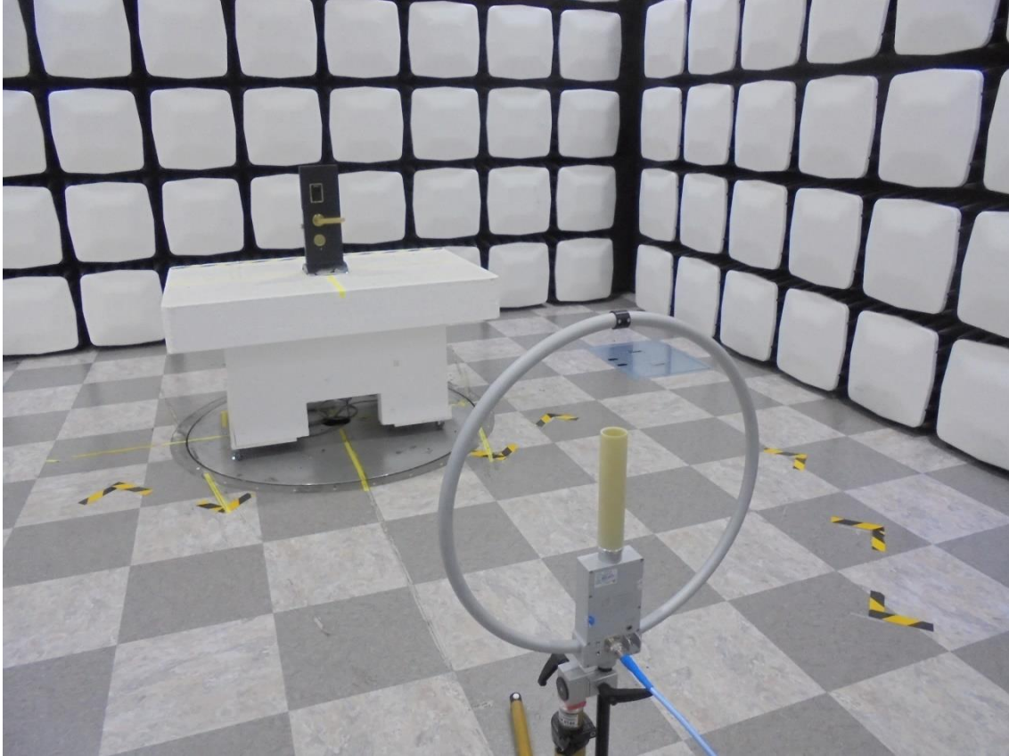
NFC Radiated Test Setup Photo for below 30 MHz:
