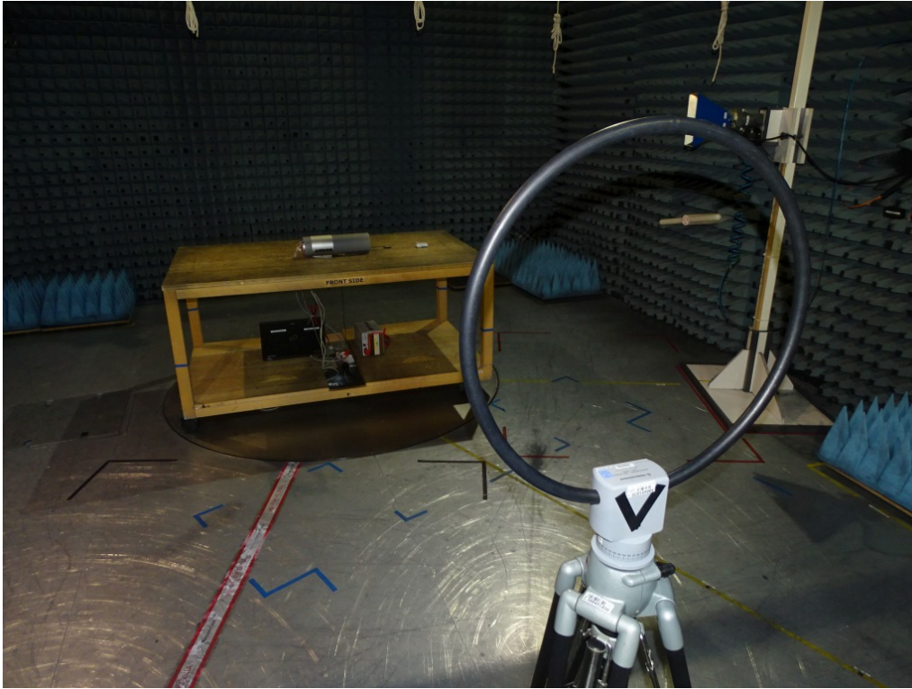
Photo 2: Test setup for radiated measurements (H-Field)
