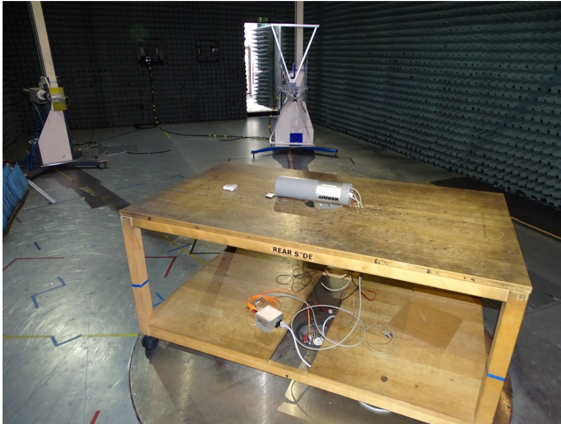
Photo 3: Test setup for radiated measurements (30 MHz – 1 GHz)
