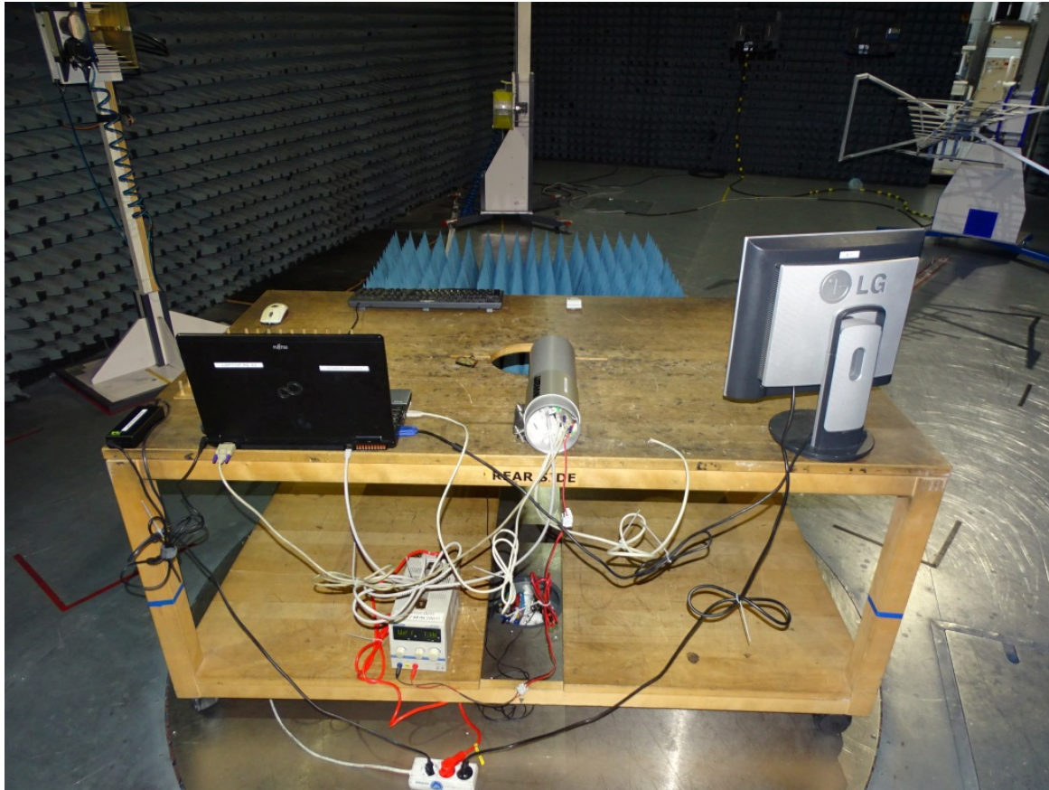
Photo 7: Test setup for radiated measurements (computer peripheral setup, above 1 GHz)
