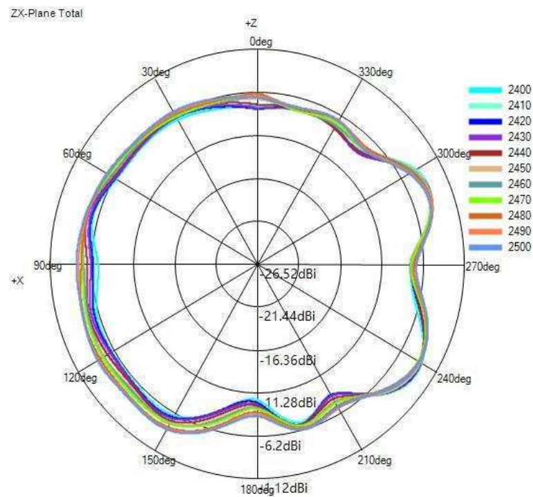
(1) X-Z Plane(unit:dBi):
