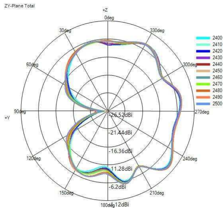
(2) Y-Z Plane(unit:dBi):
