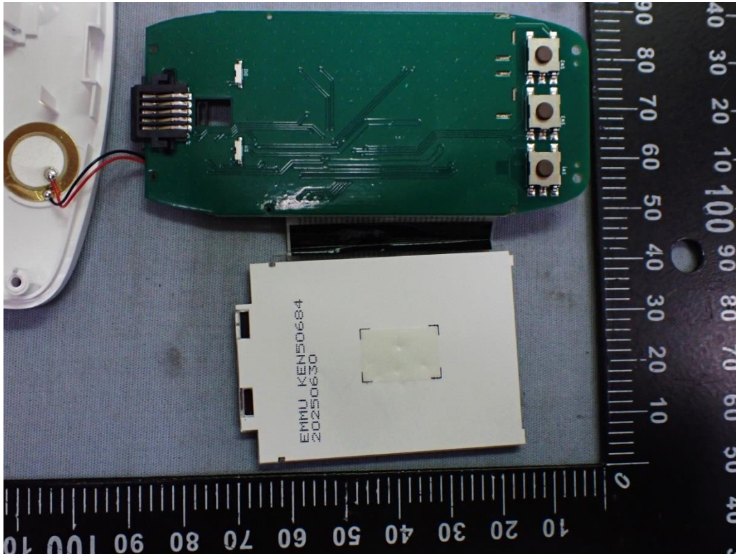
Figure 9 Internal View (Removed LCD Panel)
