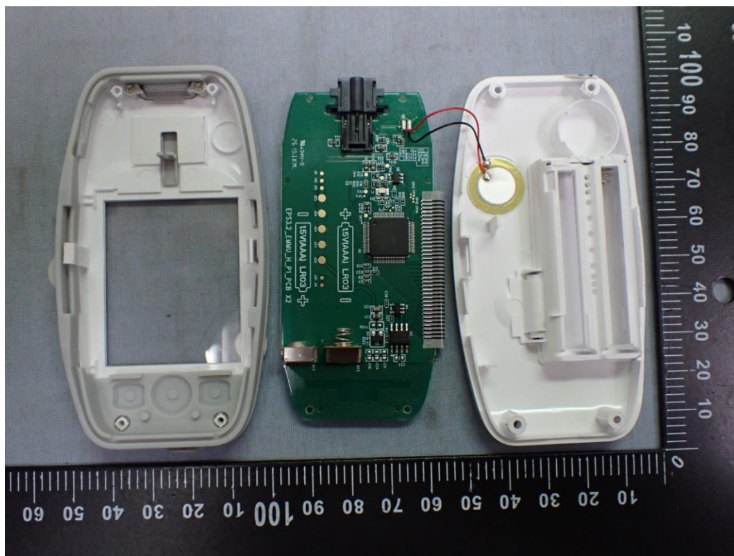
Figure 8 Internal View (Internal Board / Front View)
