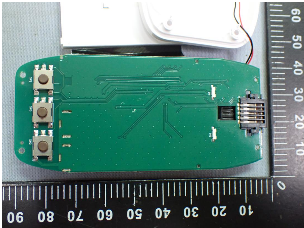
Figure 10 Internal View (Internal Board / Back View)
