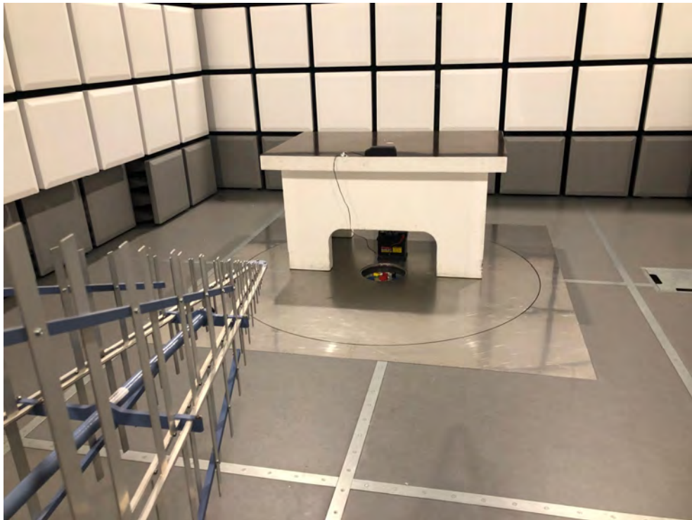
Figure 6: Radiated emission test
