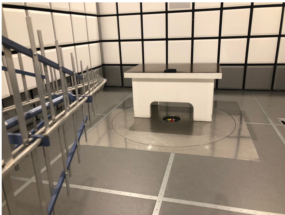
Figure 7: Radiated emission test
