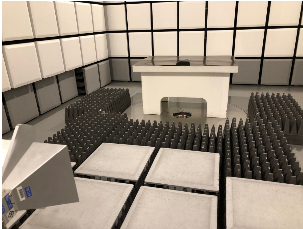
Figure 10: Radiated emission test
