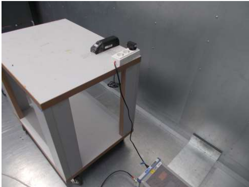
Figure 1: Conducted emission test – Charging from AC/DC power supply
