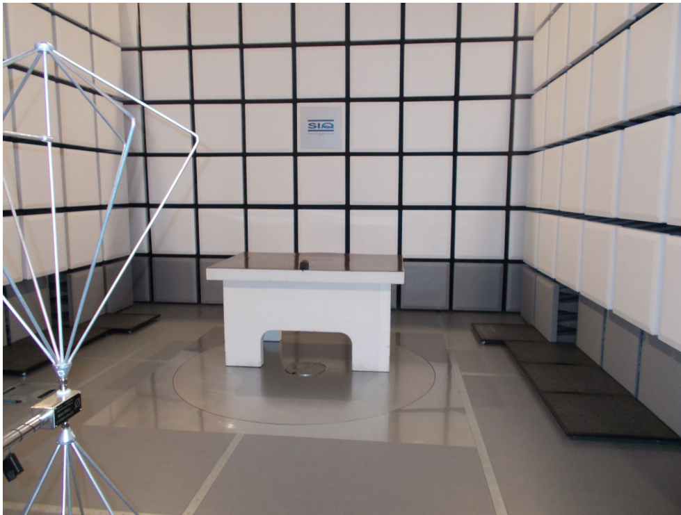
Figure 2: Radiated emission test – battery operating
