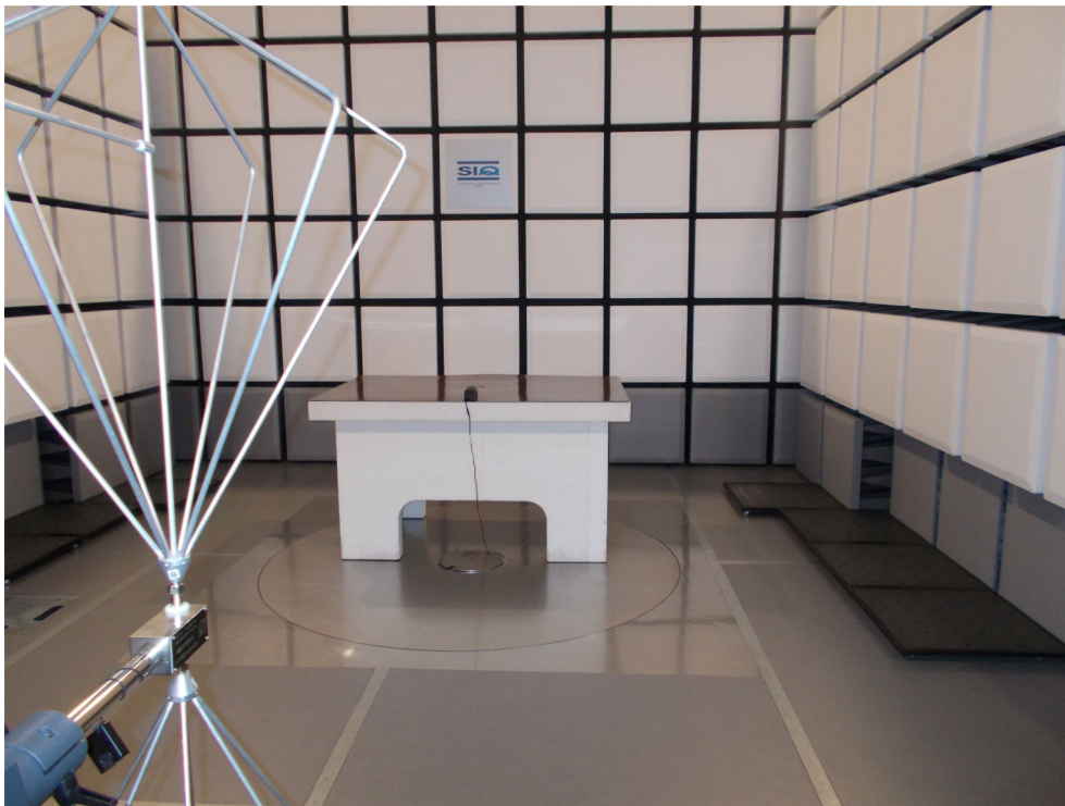
Figure 3: Radiated emission test – charging from battery power supply
