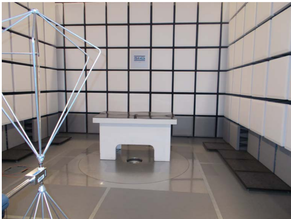
Figure 3: Radiated emission test 30 MHz – 200 MHz (without charger)
