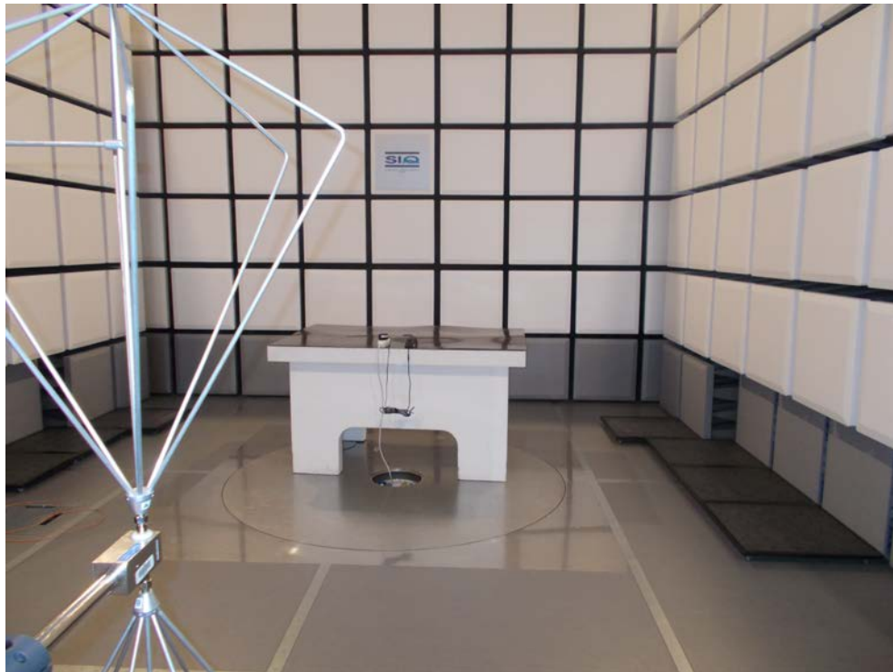
Figure 2: Radiated emission test 30 MHz – 200 MHz (with charger)
