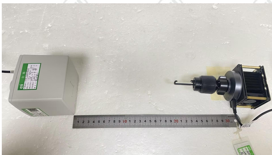
Test Setup of Bottom (Mode b to Mode d)
