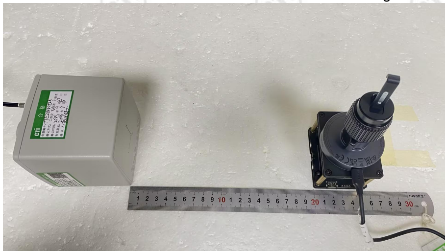
Test Setup of Left(Mode b to Mode d)
