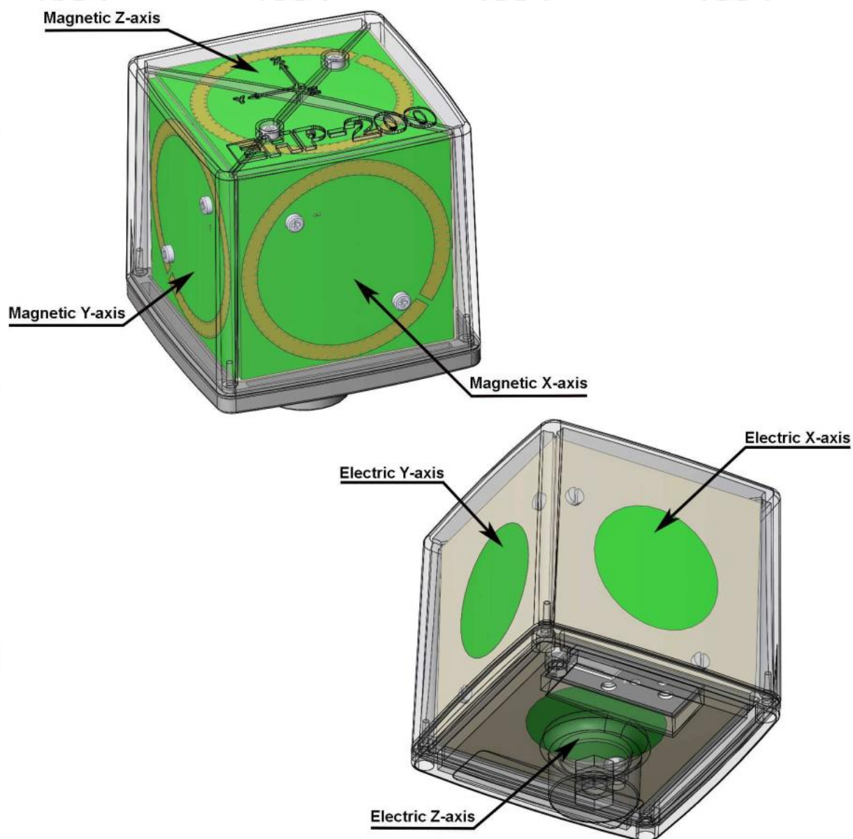
Fig. 1-4 EHP-200A/EHP-200AC axes
