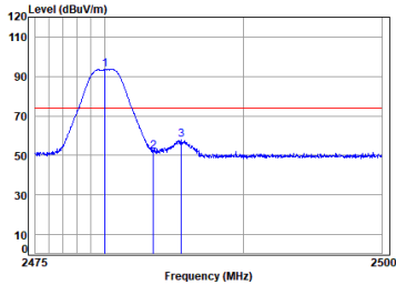
BLE_2M_TX_CH_39_Horizontal-Peak
