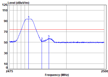
BLE_2M_TX_CH_39_Vertical-Peak
