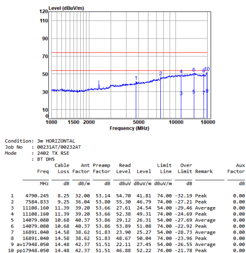
BT_DH5_TX_CH_00_Horizontal
