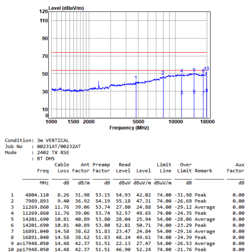
BT_DH5_TX_CH_00_Vertical
