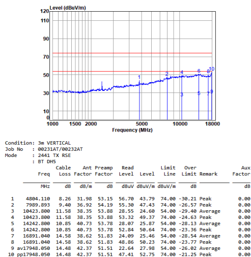
BT_DH5_TX_CH_39_Vertical
