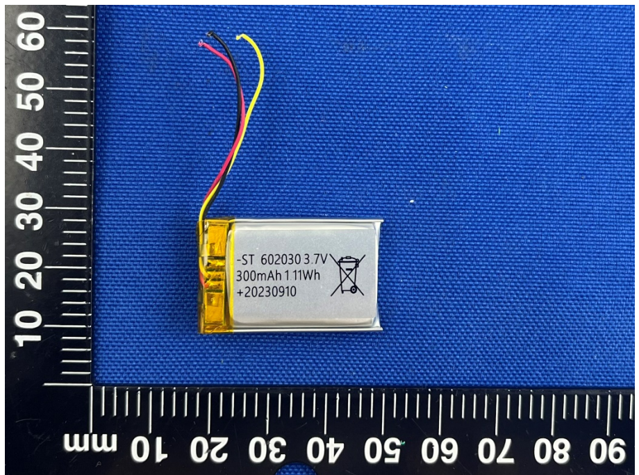
BATTERY (FRONT)
