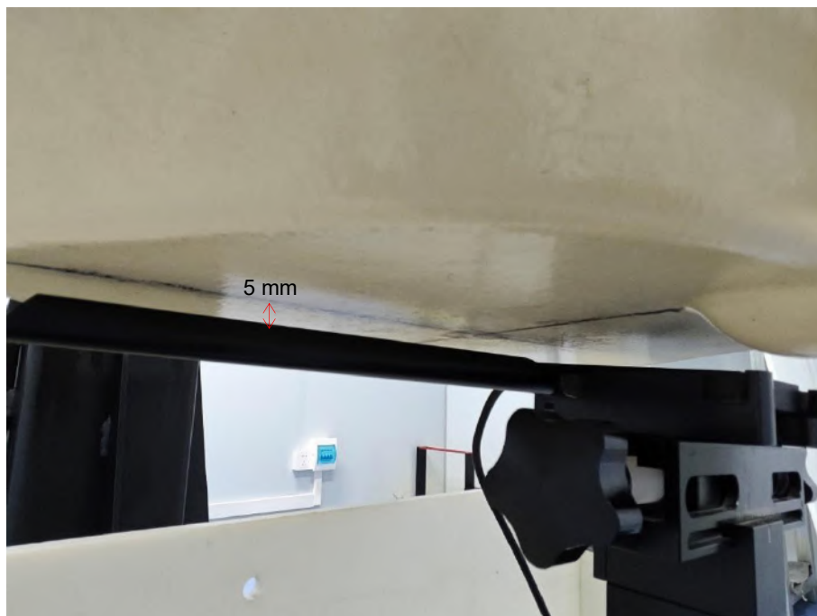
Front Side-2 (Ant.Main) (5mm)
