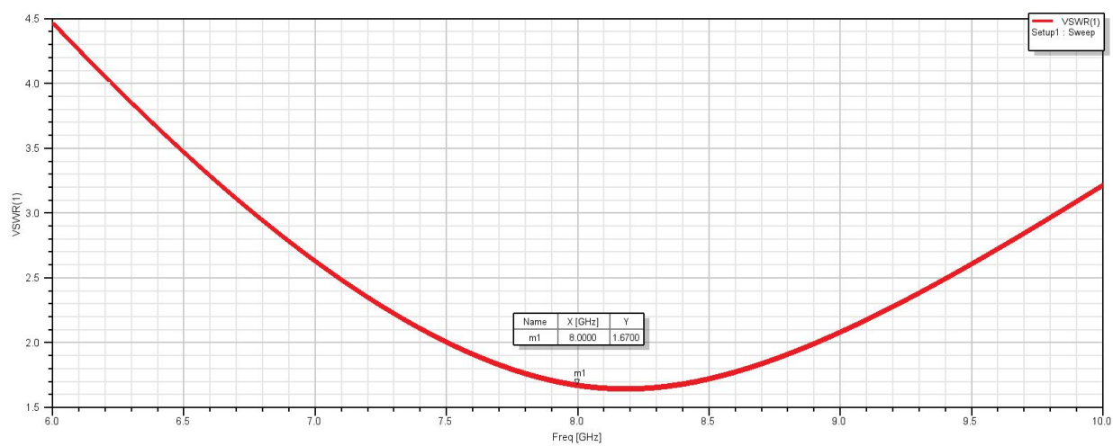
FIG. 3 Voltage Standing Wave Ratio
