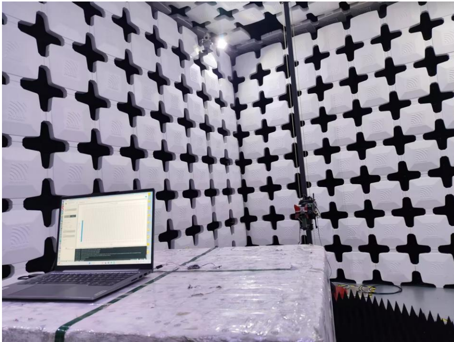
FPC Antenna 1
