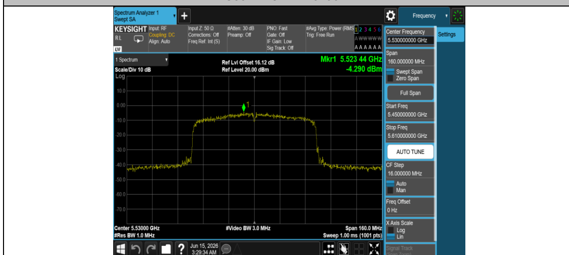
11AC80MIMO-Ant1-5530-PASS
