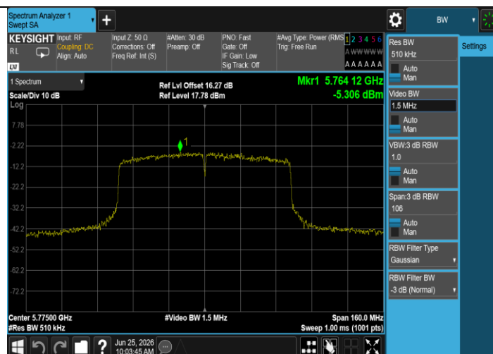
11AC80MIMO-Ant2-5775-PASS
