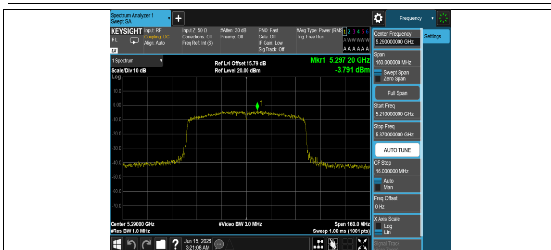
11AC80MIMO-Ant2-5290-PASS
