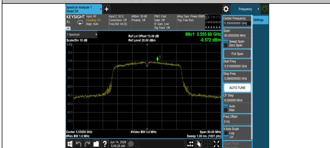
11AC40MIMO-Ant1-5550-PASS
