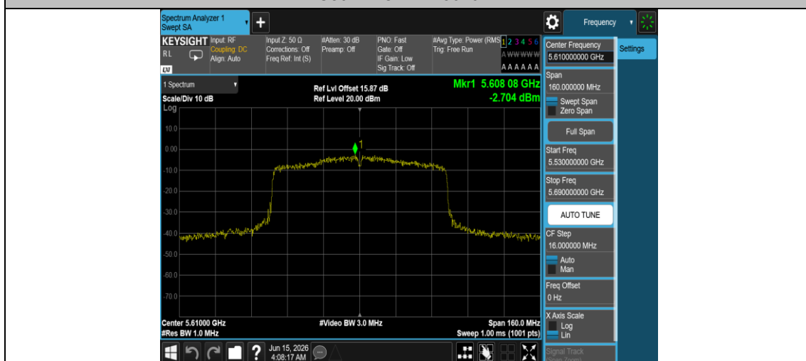
11AC80MIMO-Ant2-5610-PASS
