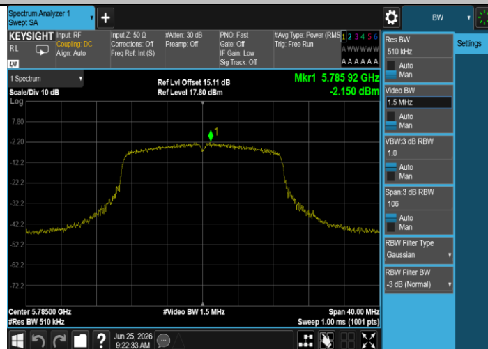
11AC20MIMO-Ant1-5785-PASS
