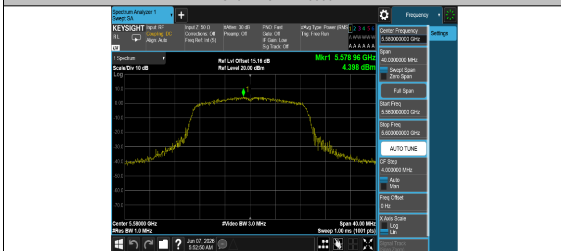
11AC20MIMO-Ant1-5580-PASS
