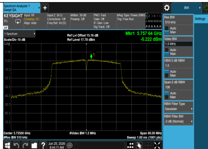
11AC40MIMO-Ant2-5755-PASS
