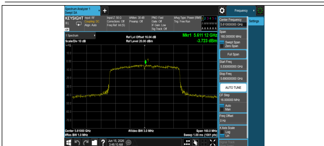
11AC80MIMO-Ant1-5610-PASS
