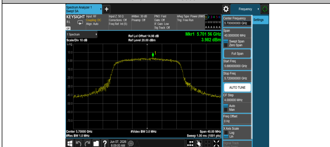
11AC20MIMO-Ant1-5700-PASS
