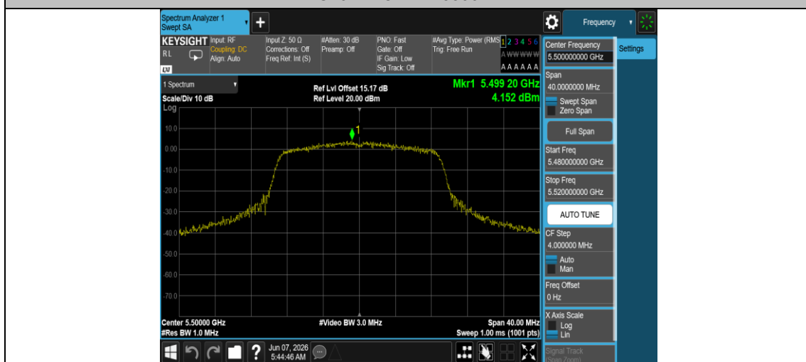
11AC20MIMO-Ant2-5500-PASS
