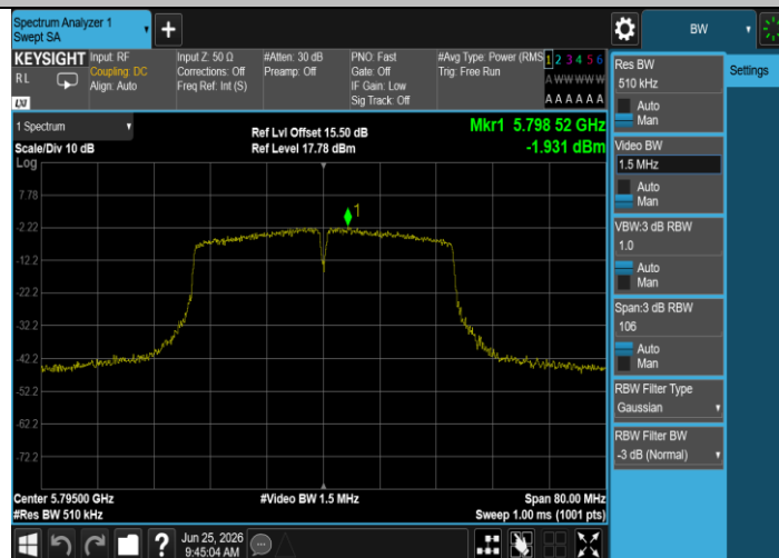
11AC40MIMO-Ant1-5795-PASS
