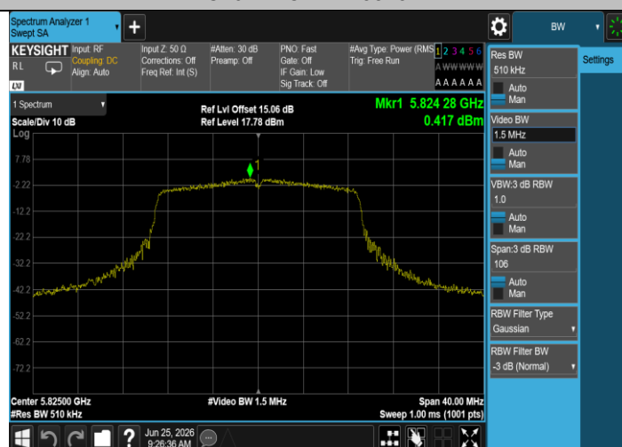
11AC20MIMO-Ant2-5825-PASS
