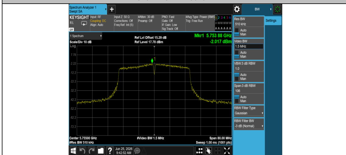
11AC40MIMO-Ant1-5755-PASS
