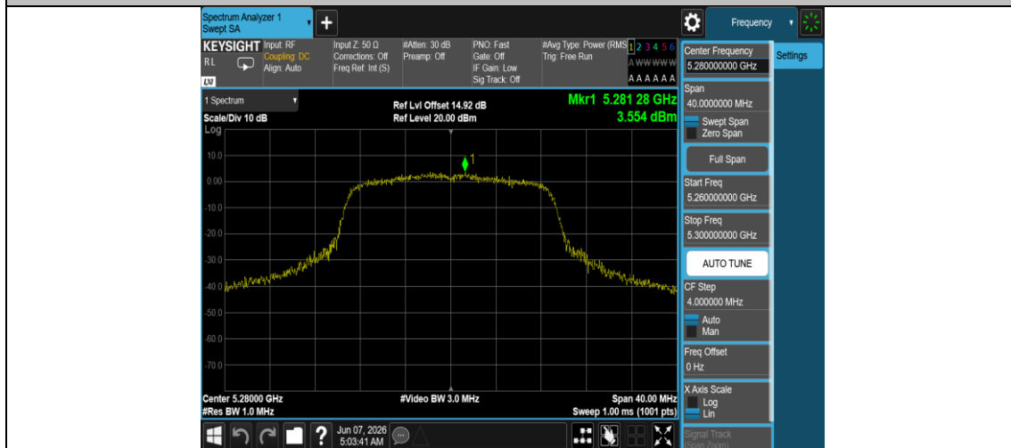
11AC20MIMO-Ant1-5280-PASS
