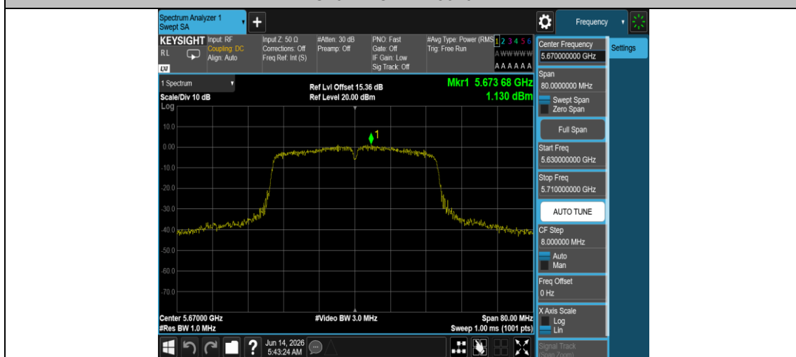
11AC40MIMO-Ant2-5670-PASS
