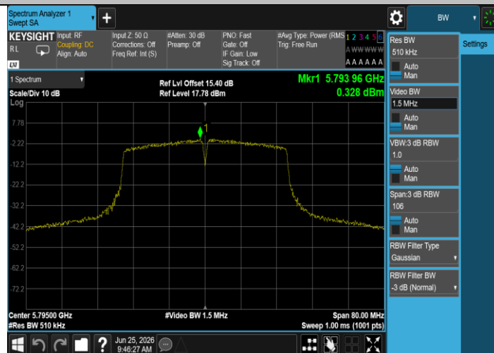
11AC40MIMO-Ant2-5795-PASS
