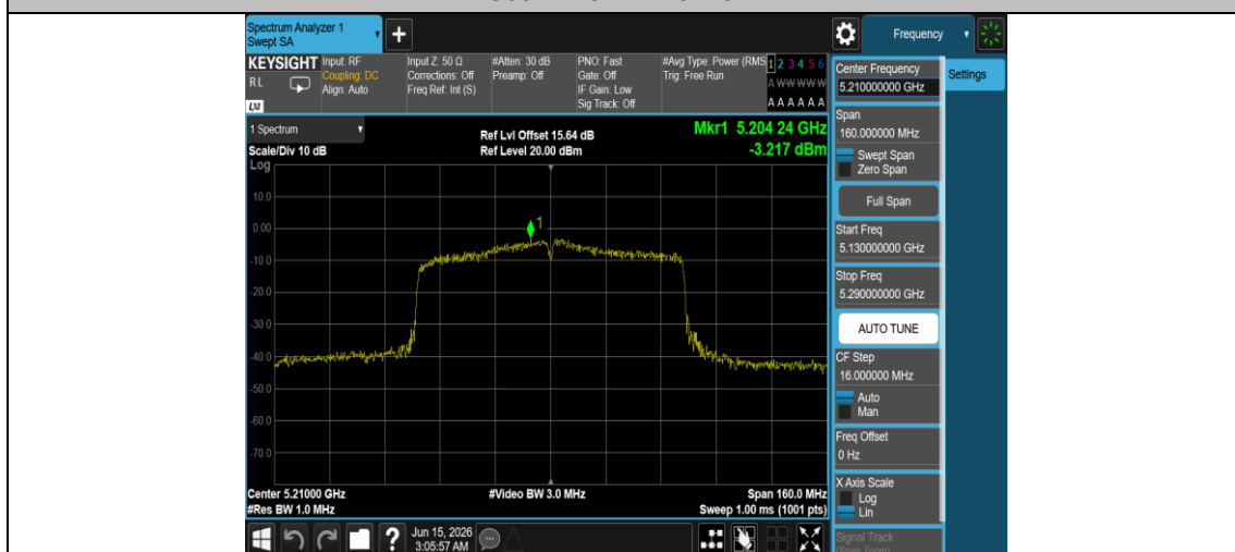
11AC80MIMO-Ant2-5210-PASS
