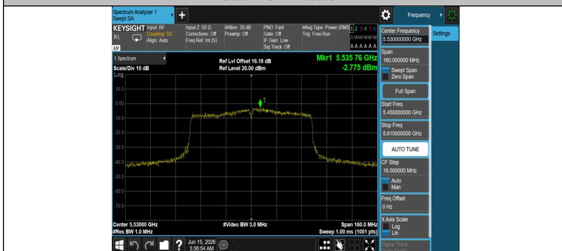
11AC80MIMO-Ant2-5530-PASS
