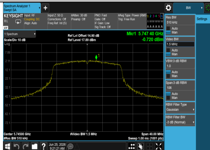
11AC20MIMO-Ant2-5745-PASS
