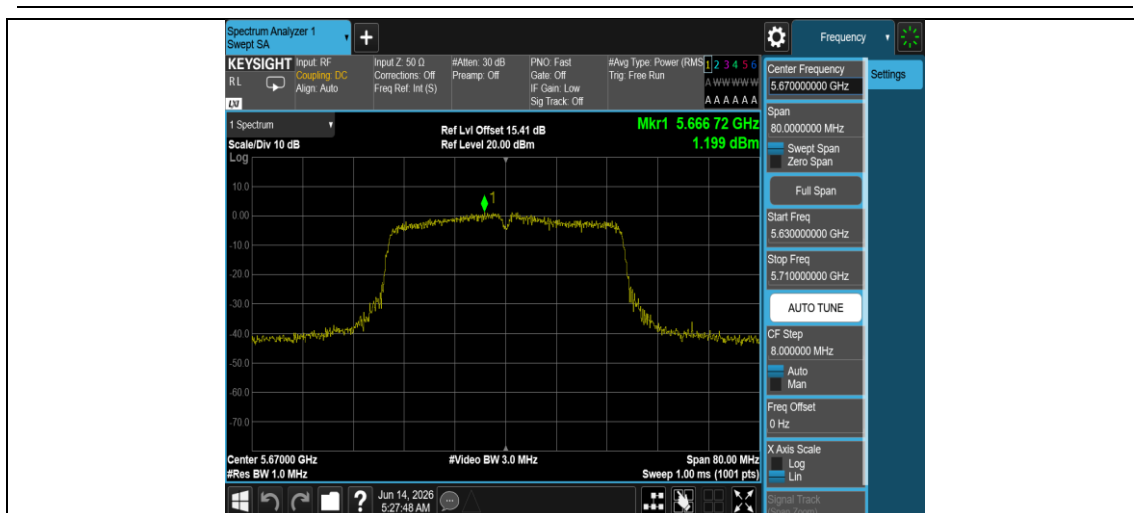
11AC40MIMO-Ant1-5670-PASS
