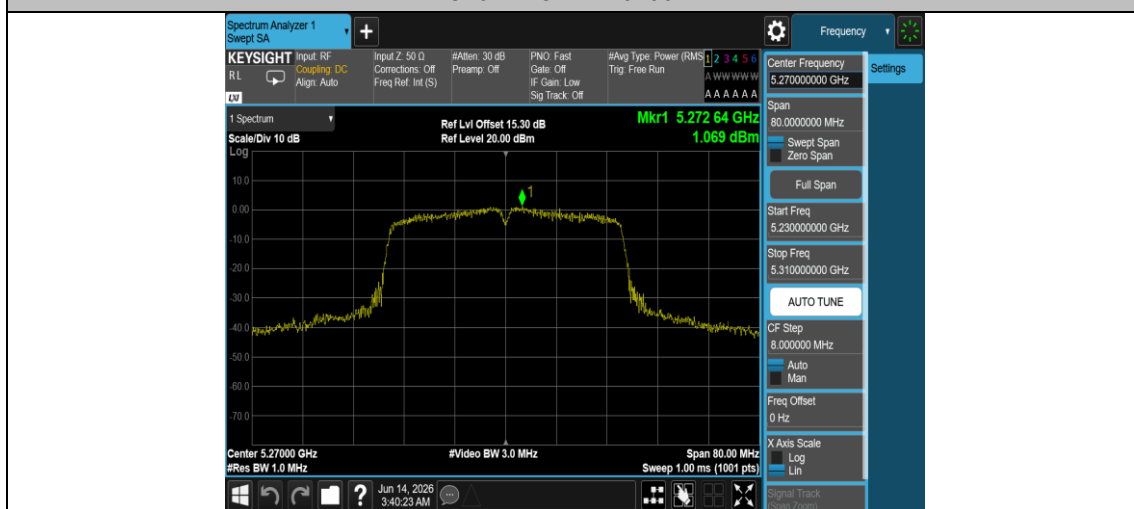
11AC40MIMO-Ant1-5270-PASS
