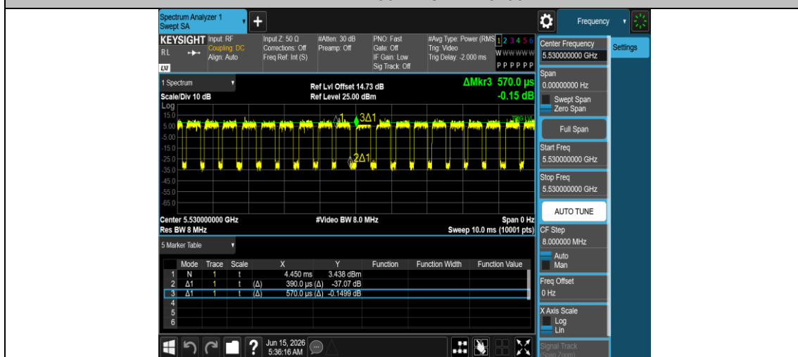
NTNV-11AX80MIMO-Ant1-5530
