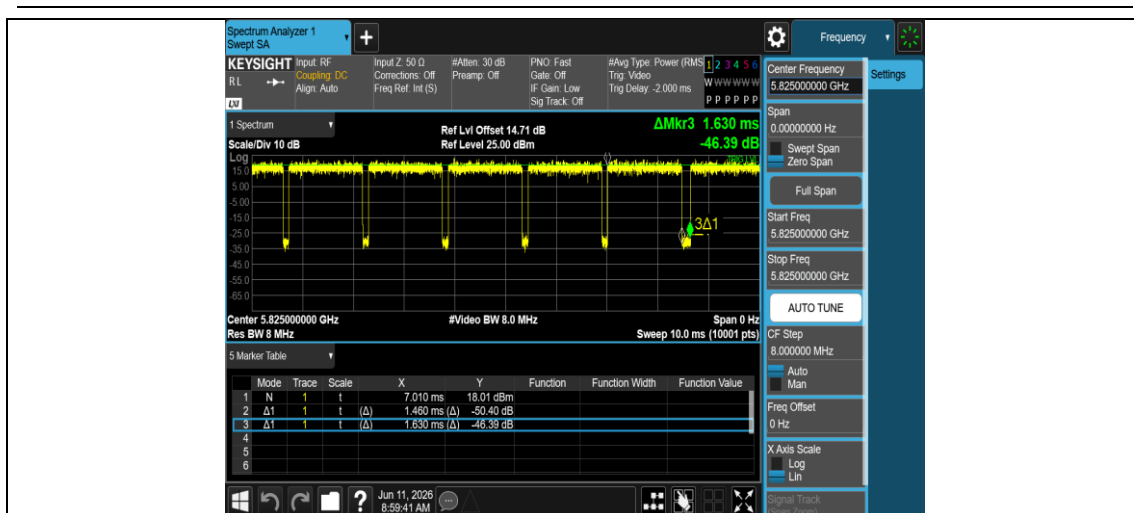
NTNV-11AX20MIMO-Ant2-5825
