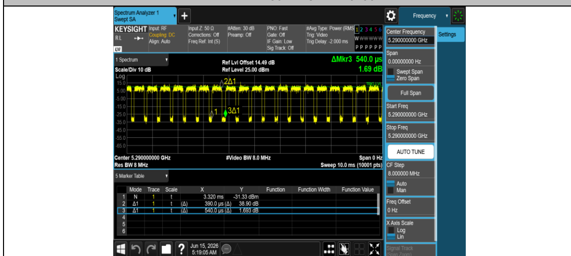
NTNV-11AX80MIMO-Ant2-5290
