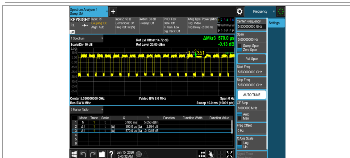
NTNV-11AX80MIMO-Ant2-5530
