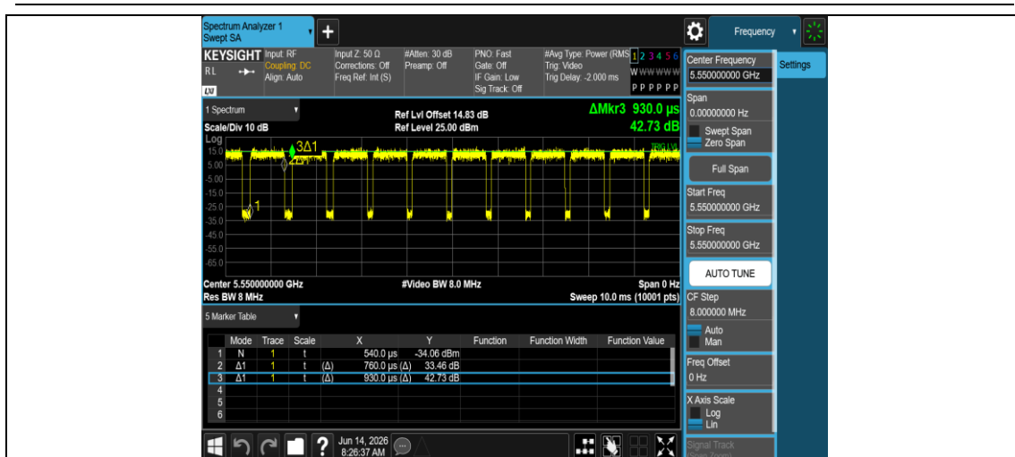
NTNV-11AX40MIMO-Ant2-5550
