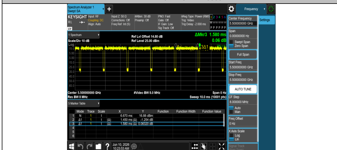
NTNV-11AX20MIMO-Ant2-5500
