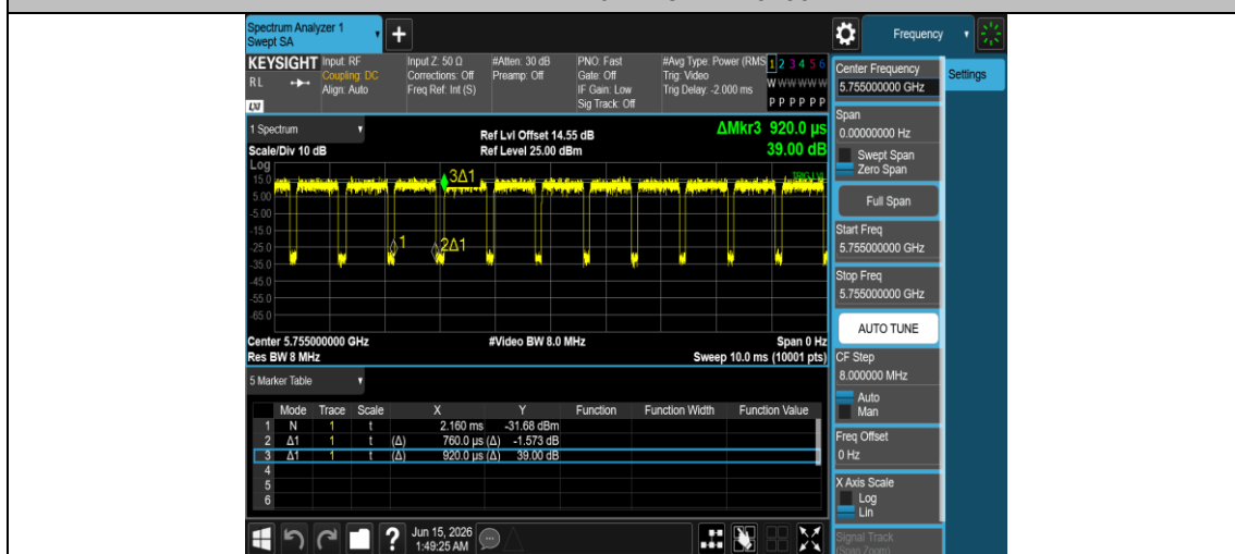
NTNV-11AX40MIMO-Ant2-5755
