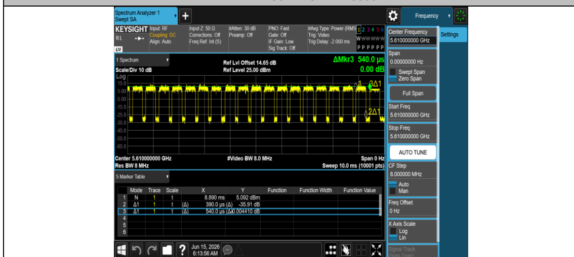
NTNV-11AX80MIMO-Ant1-5610
