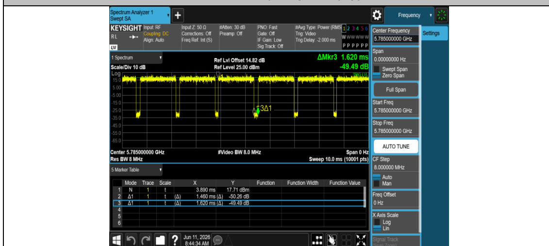
NTNV-11AX20MIMO-Ant2-5785
