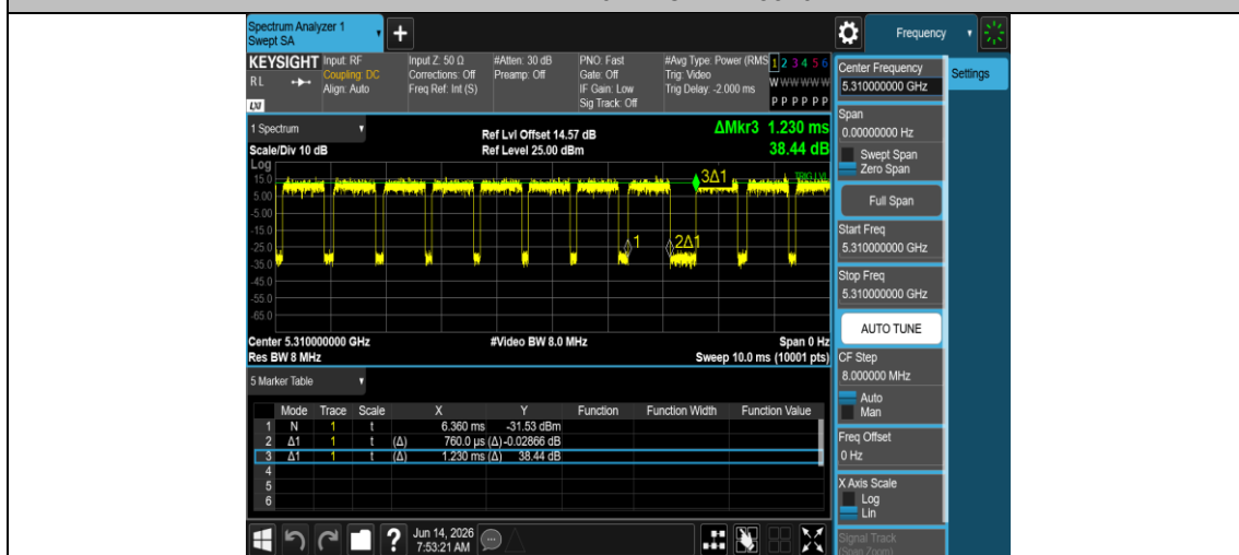
NTNV-11AX40MIMO-Ant2-5310
