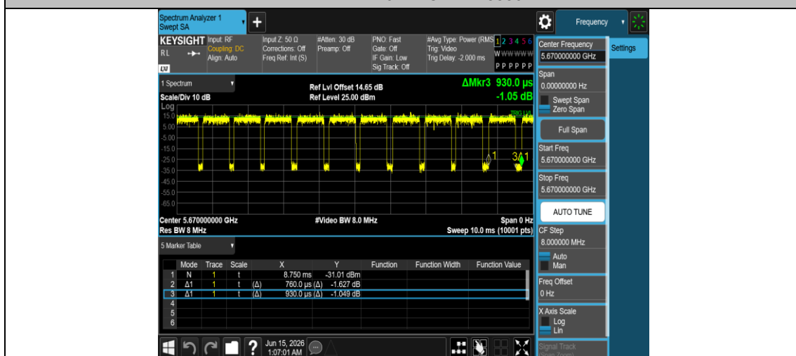
NTNV-11AX40MIMO-Ant1-5670
