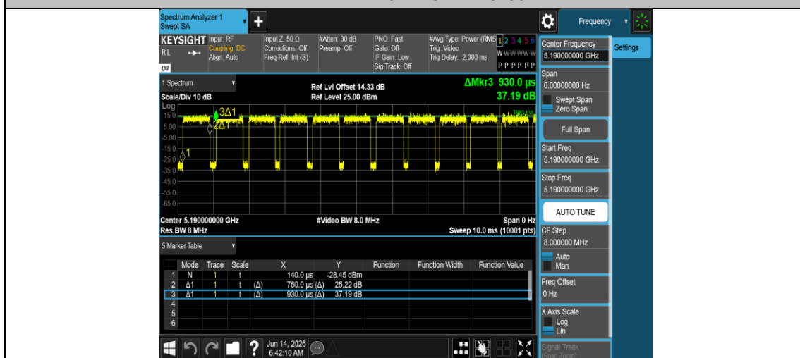
NTNV-11AX40MIMO-Ant2-5190
