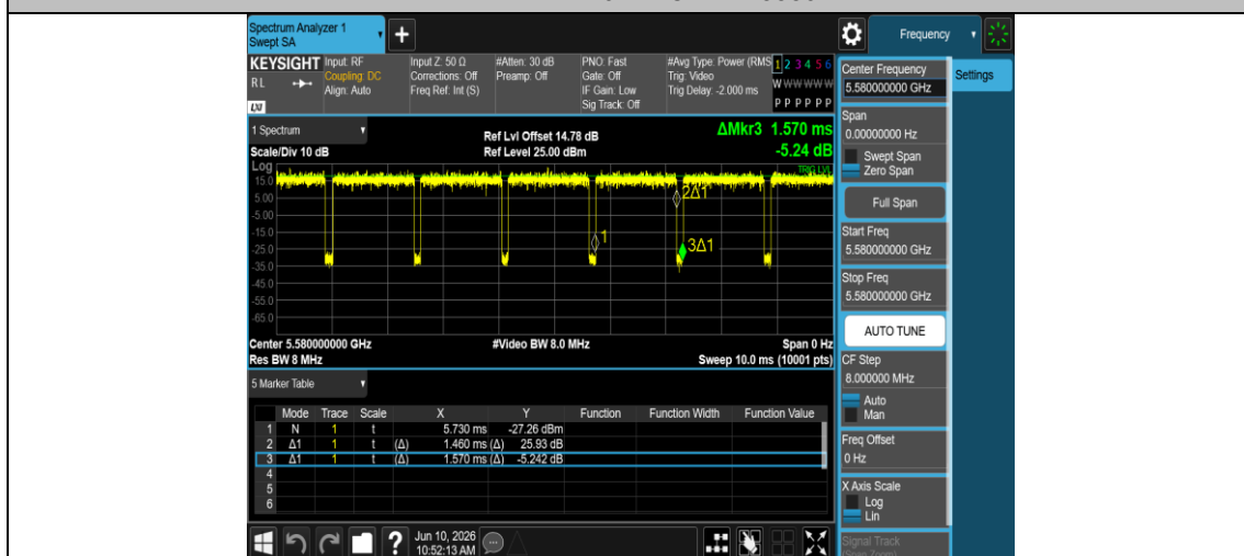
NTNV-11AX20MIMO-Ant2-5580
