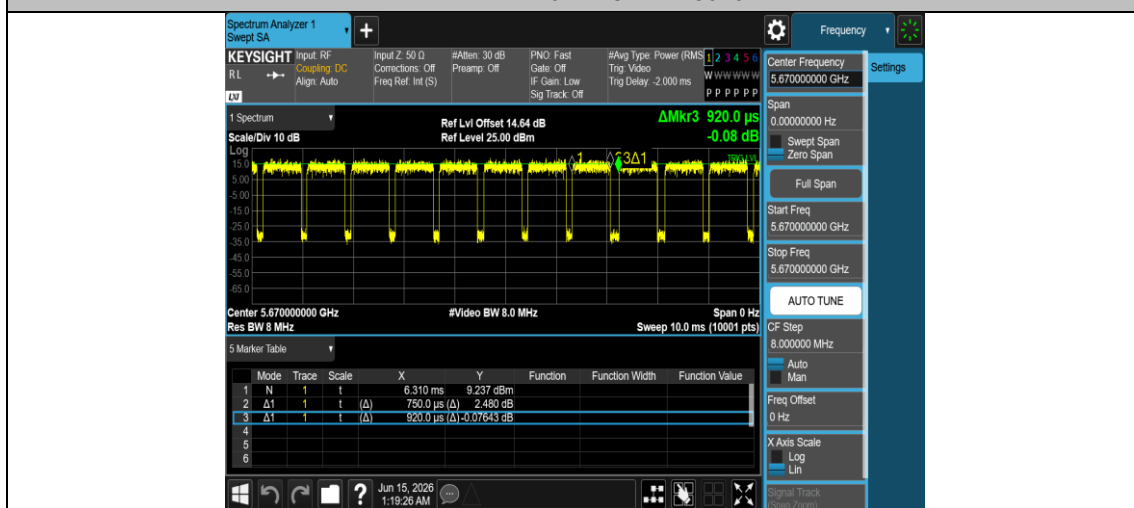
NTNV-11AX40MIMO-Ant2-5670
