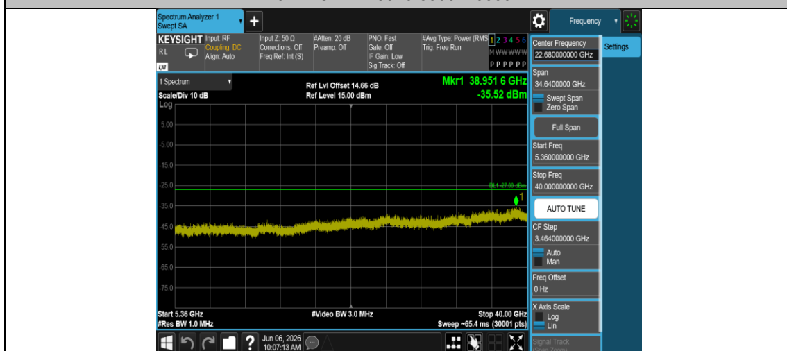
11N20MIMO-Ant2-5320-5360~40000-PASS
