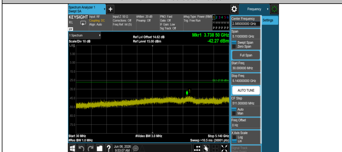
11N20MIMO-Ant1-5320-30~5140-PASS
