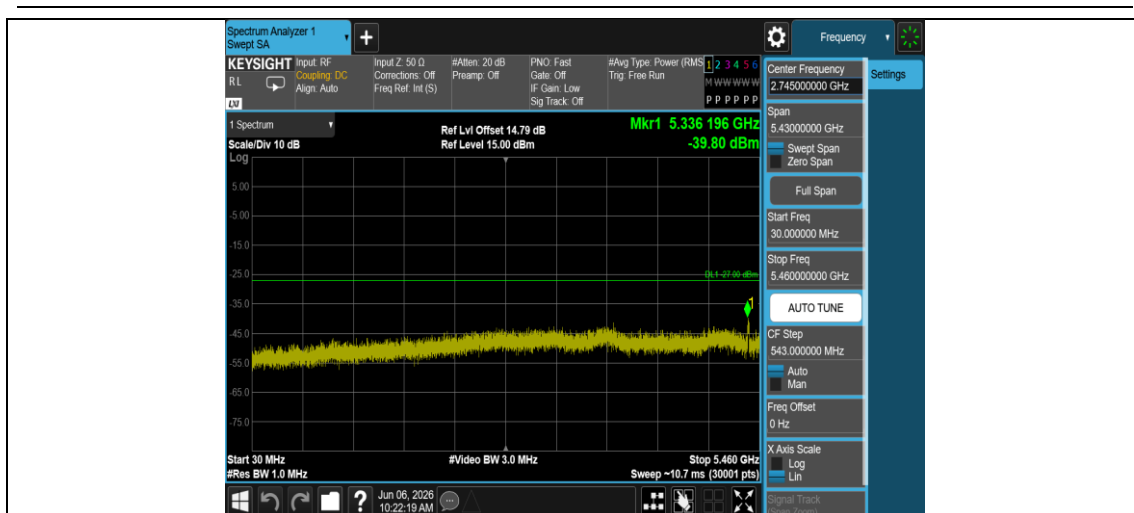
11N20MIMO-Ant1-5500-30~5460-PASS
