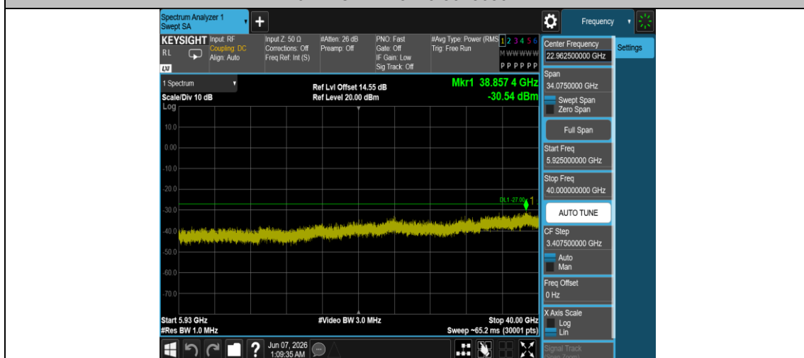
11N20MIMO-Ant1-5745-5925~40000-PASS
