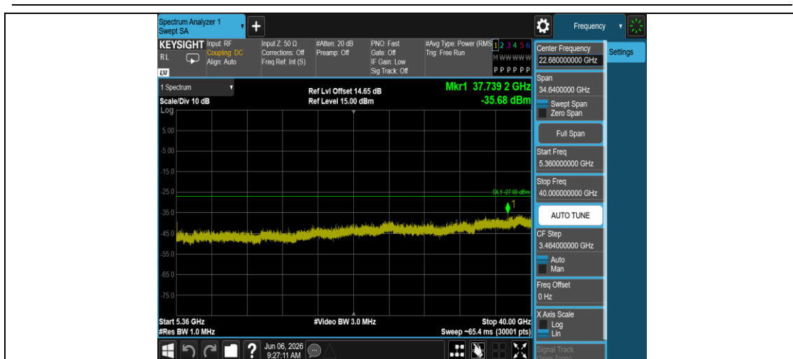
11N20MIMO-Ant1-5280-5360~40000-PASS
