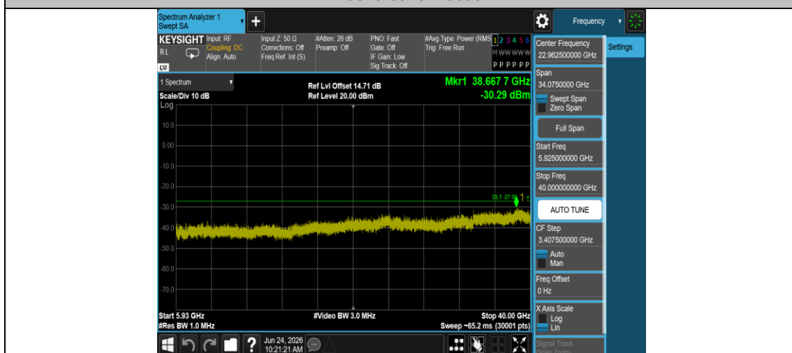
11A-Ant2-5825-5925~40000-PASS
