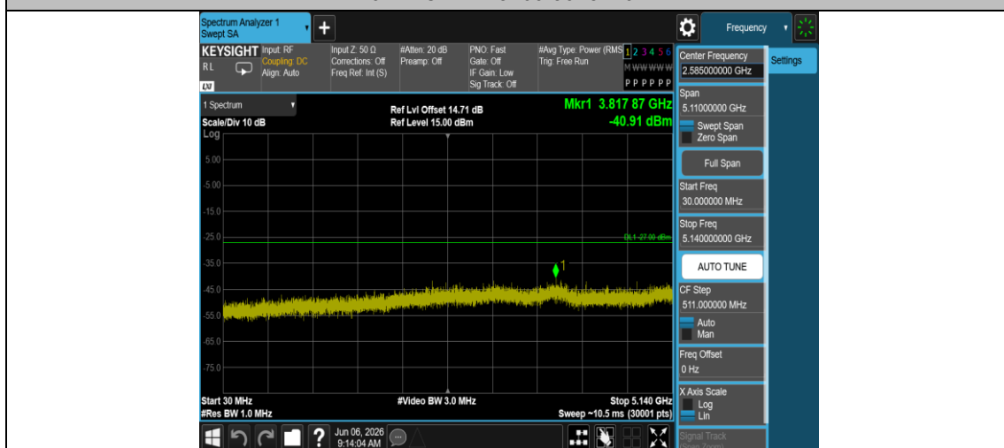
11N20MIMO-Ant2-5260-30~5140-PASS
