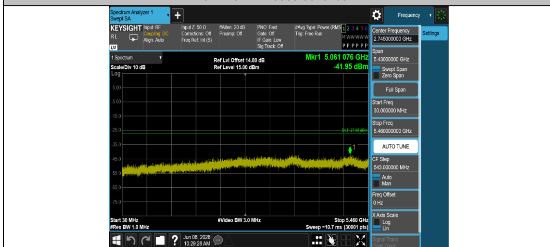
11N20MIMO-Ant2-5500-30~5460-PASS
