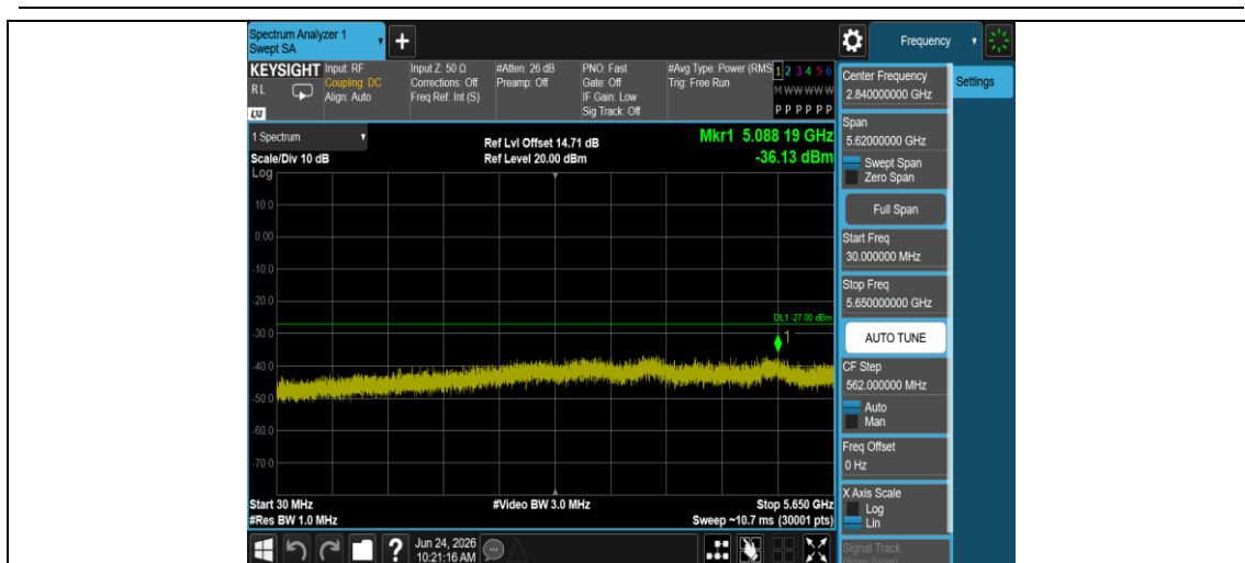
11A-Ant2-5825-30~5650-PASS
