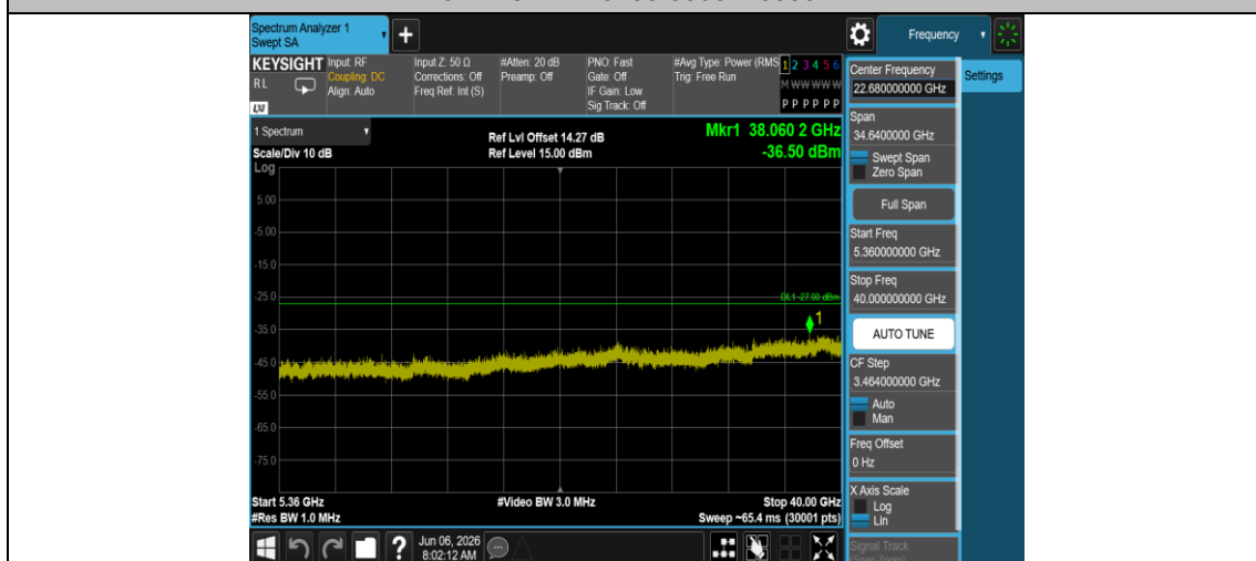
11N20MIMO-Ant2-5200-5360~40000-PASS
