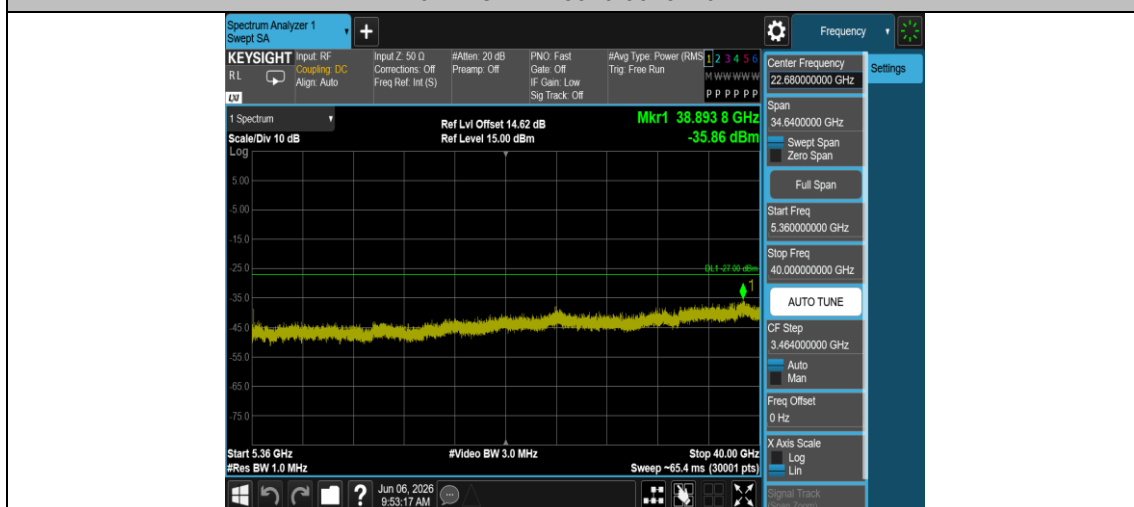
11N20MIMO-Ant1-5320-5360~40000-PASS
