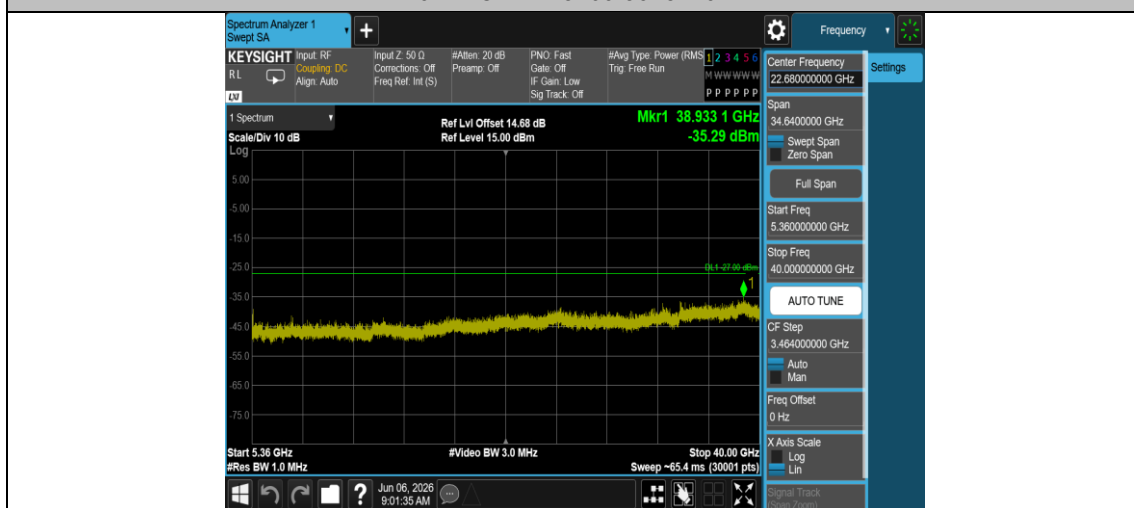
11N20MIMO-Ant1-5260-5360~40000-PASS
