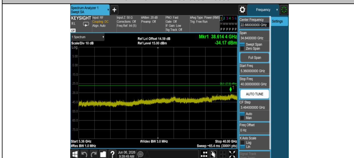
11N20MIMO-Ant2-5280-5360~40000-PASS
