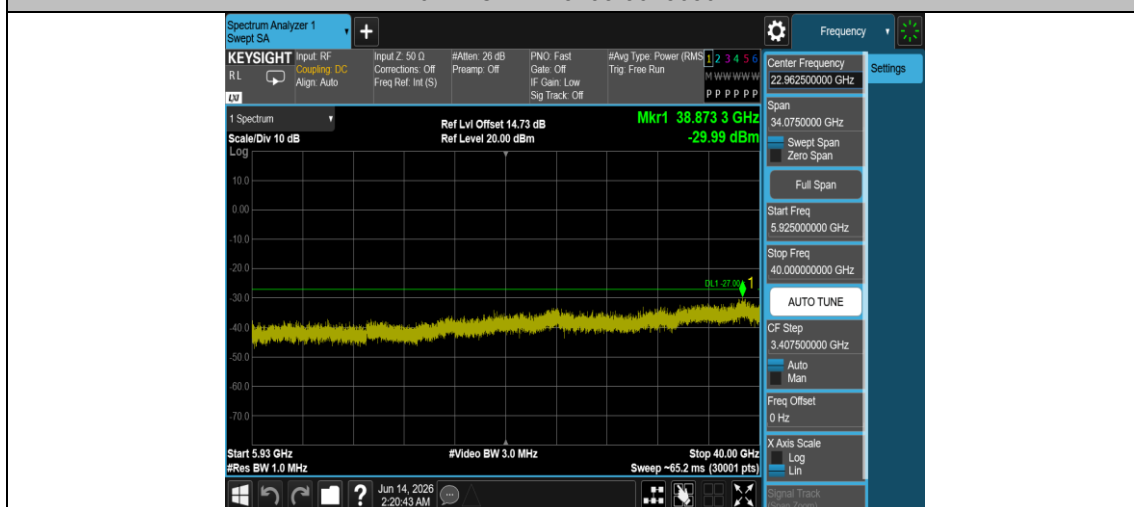
11N40MIMO-Ant1-5795-5925~40000-PASS
