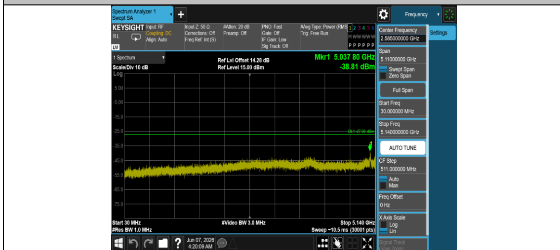
11AC20MIMO-Ant1-5200-30~5140-PASS
