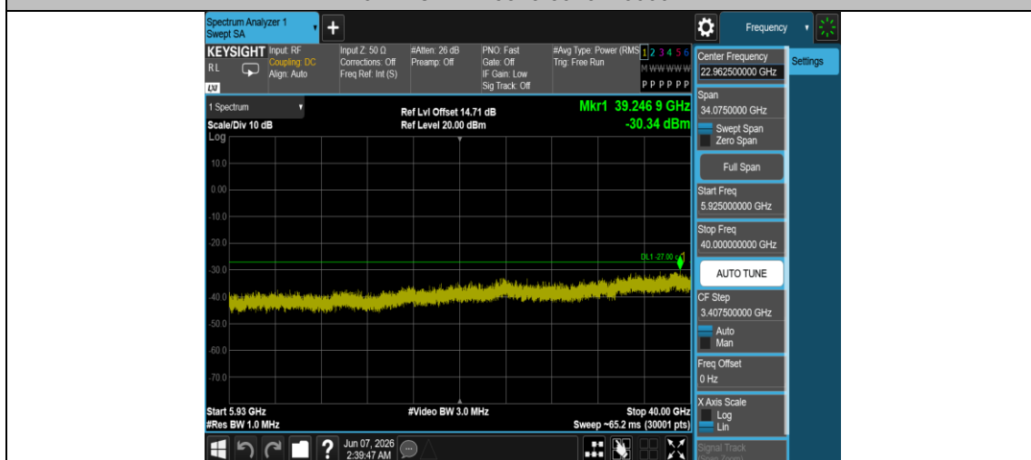
11N20MIMO-Ant2-5825-5925~40000-PASS
