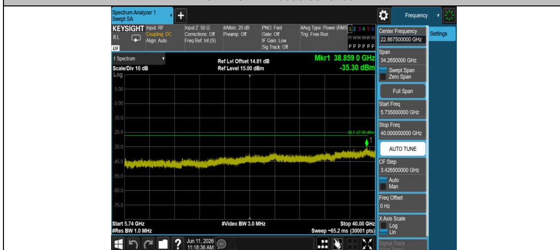
11N40MIMO-Ant1-5550-5735~40000-PASS
