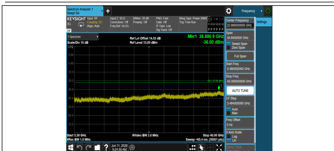
11N40MIMO-Ant1-5230-5360~40000-PASS
