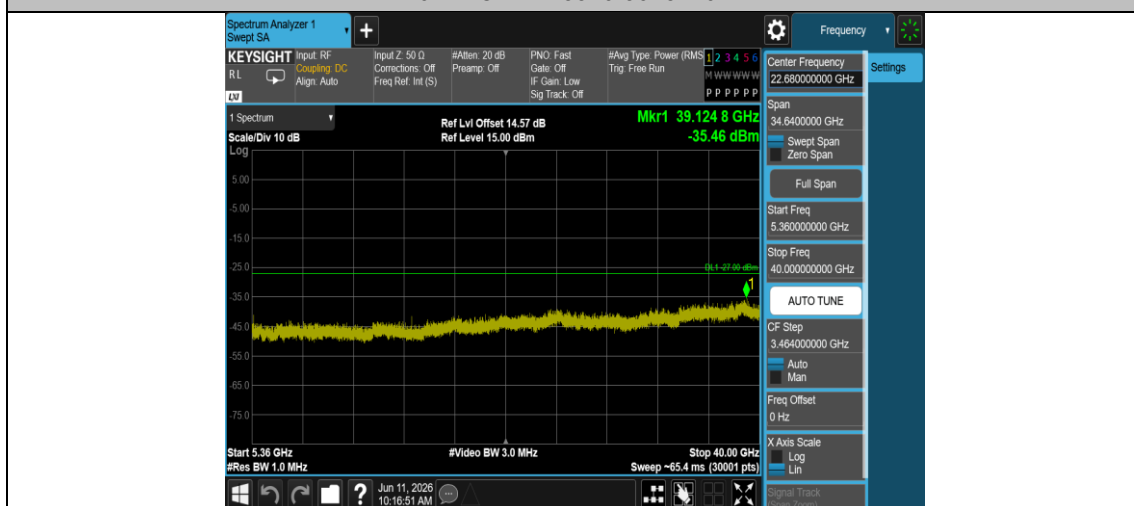
11N40MIMO-Ant1-5310-5360~40000-PASS
