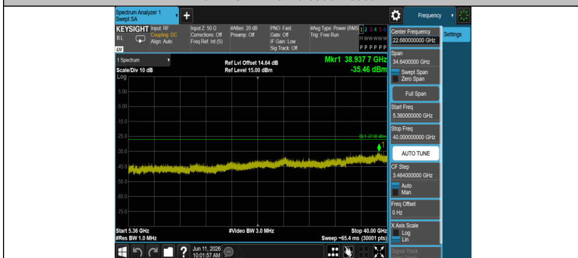
11N40MIMO-Ant2-5270-5360~40000-PASS
