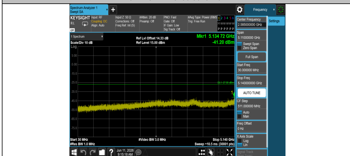
11N40MIMO-Ant2-5190-30~5140-PASS
