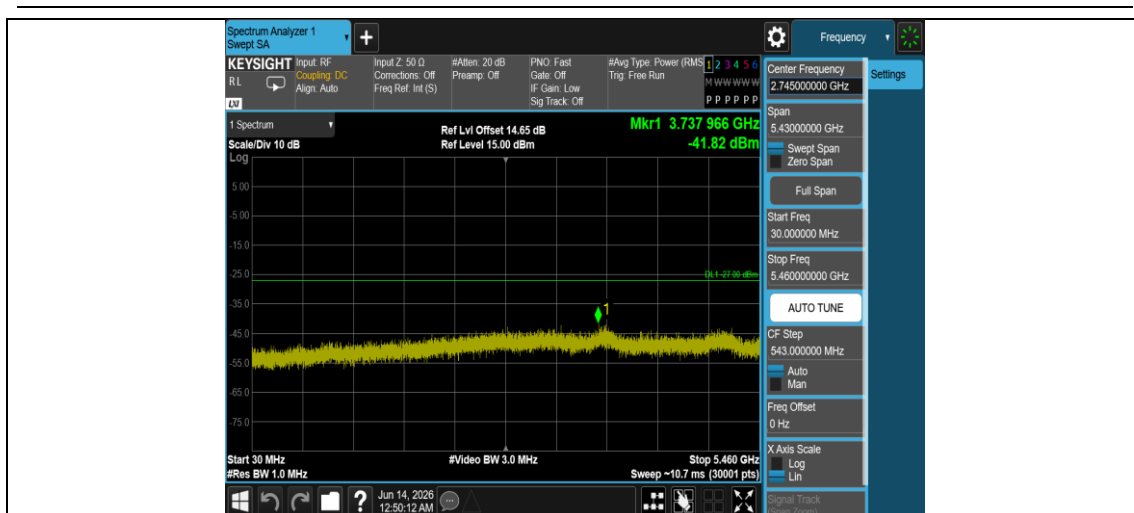
11N40MIMO-Ant1-5670-30~5460-PASS
