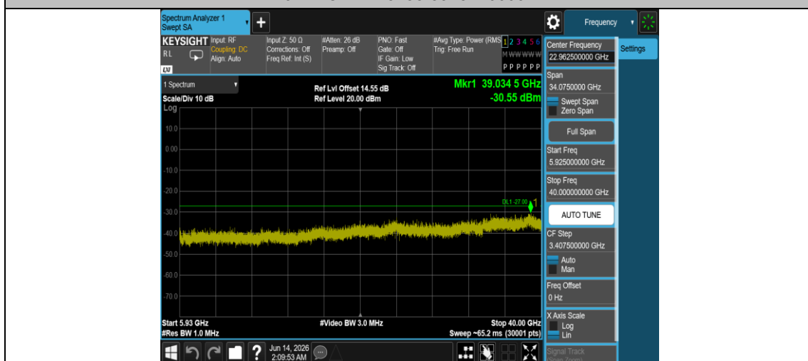
11N40MIMO-Ant2-5755-5925~40000-PASS
