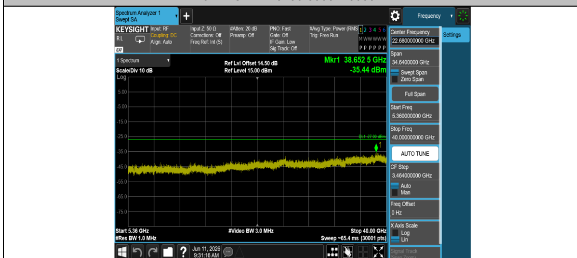
11N40MIMO-Ant2-5230-5360~40000-PASS
