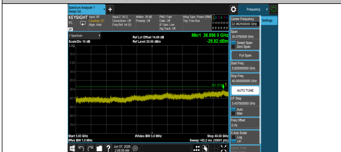
11N20MIMO-Ant1-5825-5925~40000-PASS
