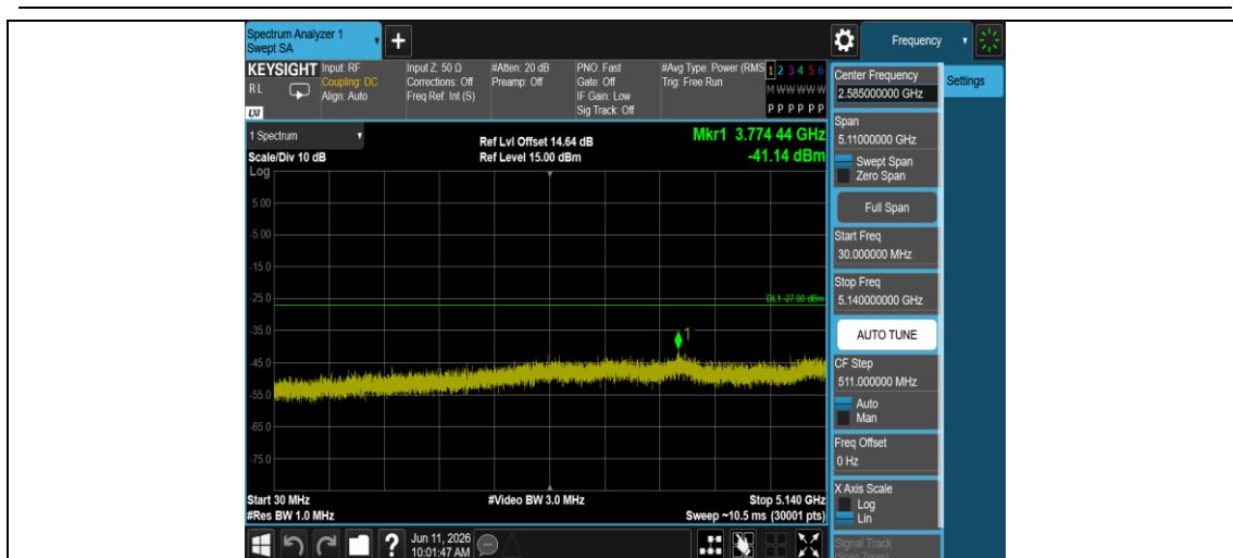
11N40MIMO-Ant2-5270-30~5140-PASS
