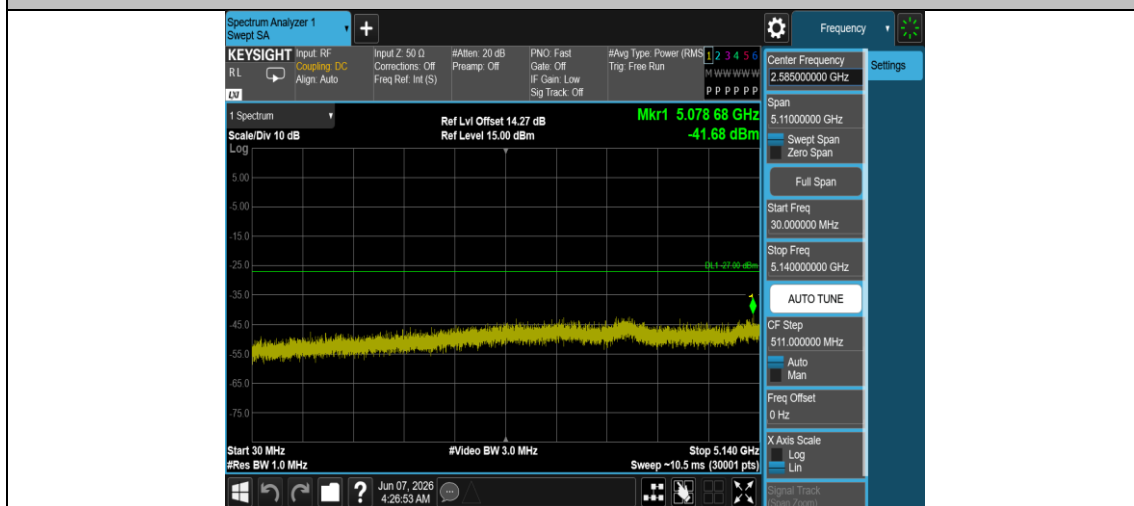
11AC20MIMO-Ant2-5200-30~5140-PASS
