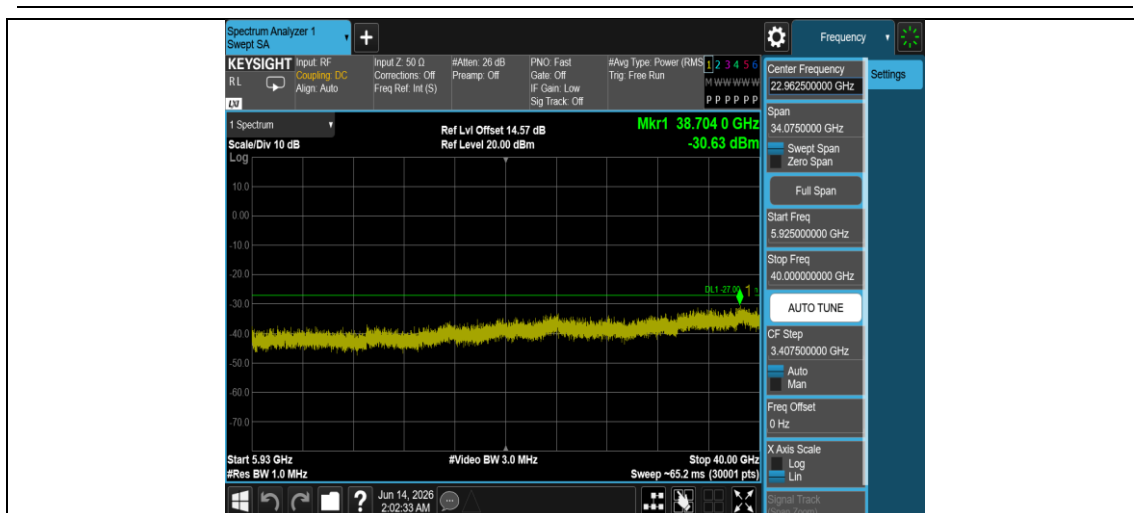
11N40MIMO-Ant1-5755-5925~40000-PASS
