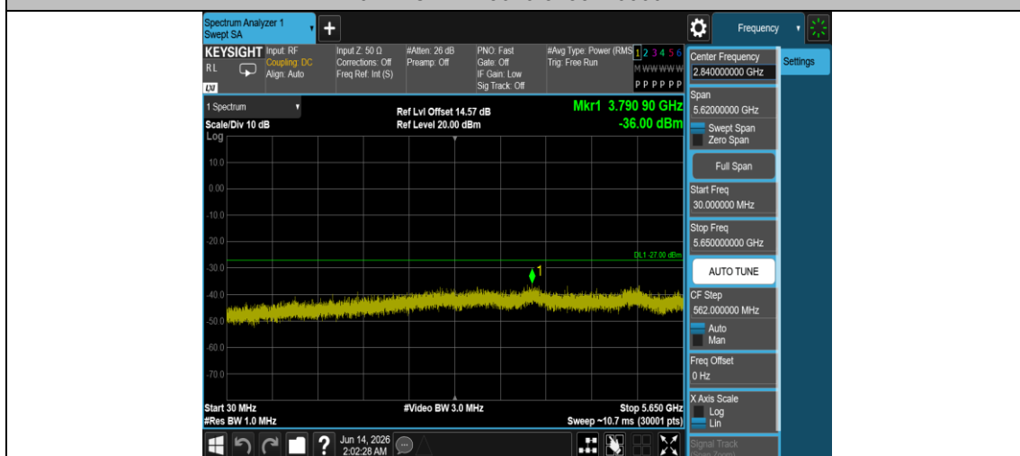
11N40MIMO-Ant1-5755-30~5650-PASS
