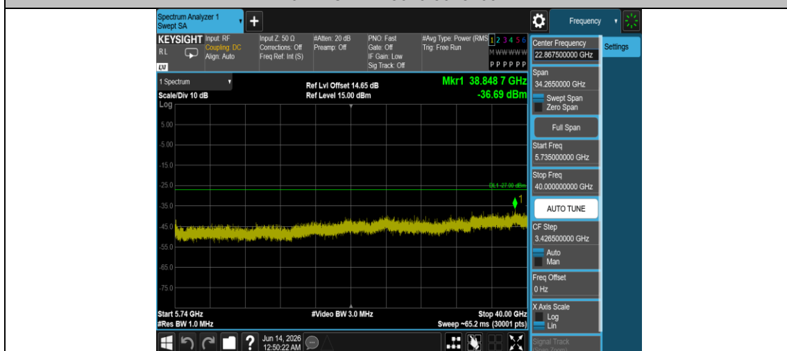
11N40MIMO-Ant1-5670-5735~40000-PASS
