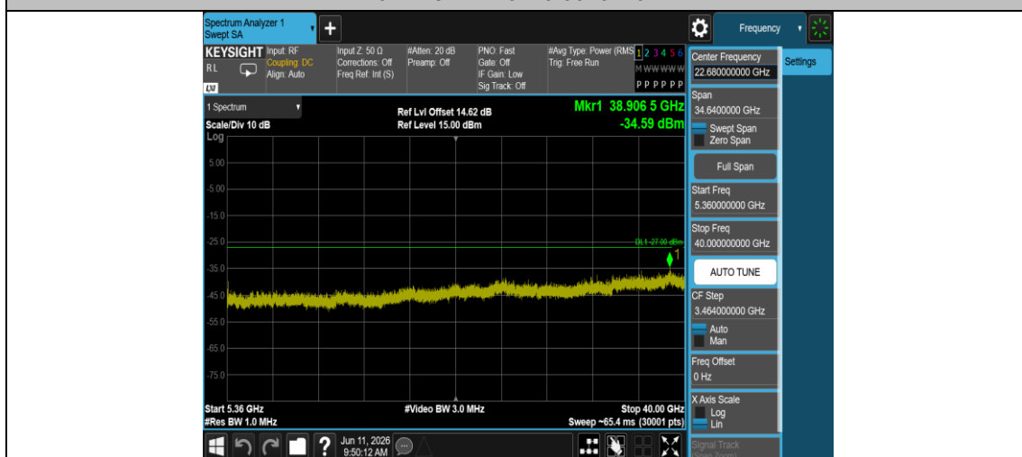
11N40MIMO-Ant1-5270-5360~40000-PASS
