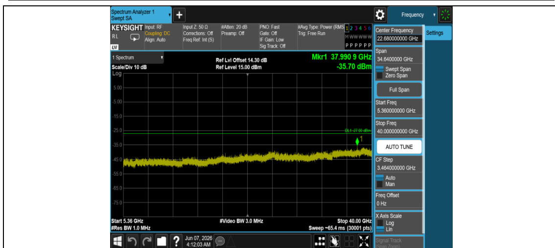
11AC20MIMO-Ant2-5180-5360~40000-PASS
