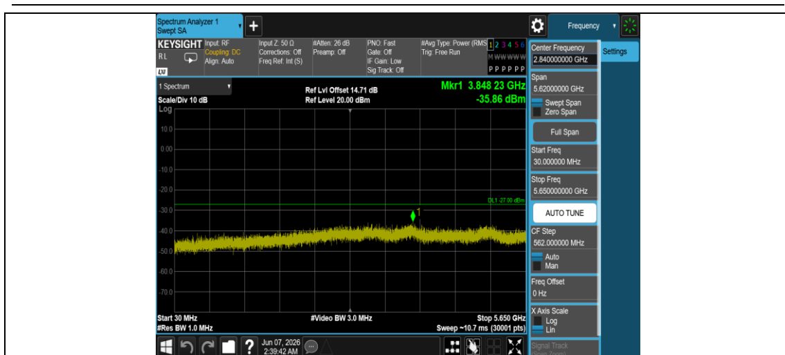
11N20MIMO-Ant2-5825-30~5650-PASS
