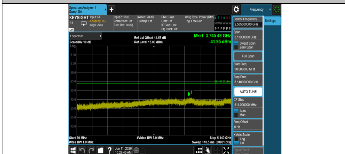
11N40MIMO-Ant2-5310-30~5140-PASS
