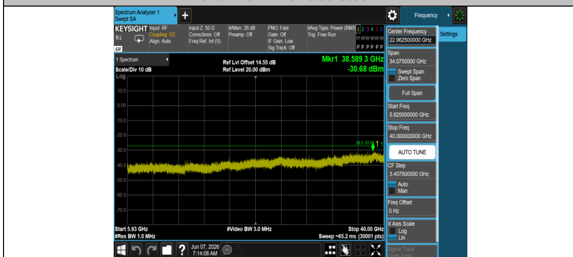
11AC20MIMO-Ant1-5745-5925~40000-PASS
