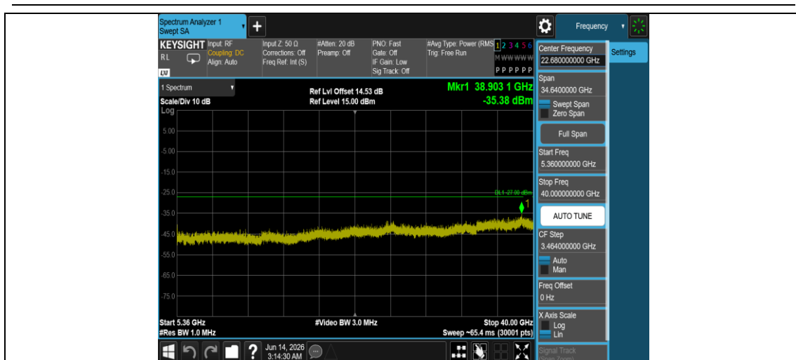
11AC40MIMO-Ant1-5230-5360~40000-PASS
