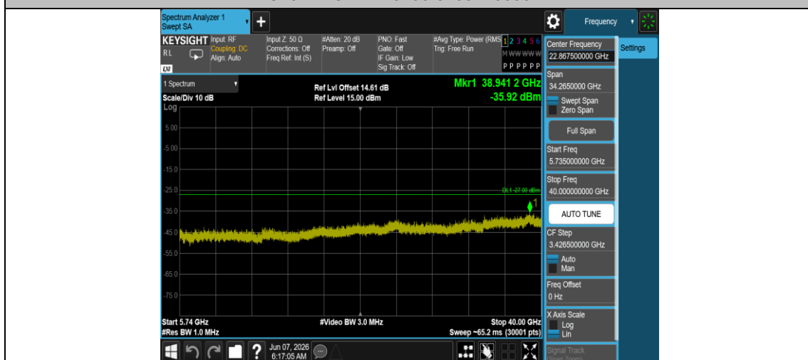
11AC20MIMO-Ant2-5700-5735~40000-PASS
