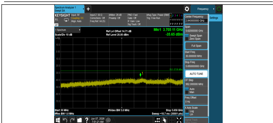
11AC20MIMO-Ant2-5825-30~5650-PASS
