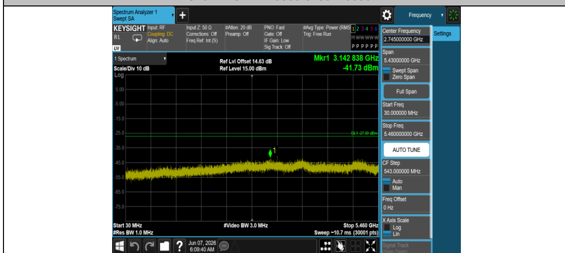
11AC20MIMO-Ant1-5700-30~5460-PASS
