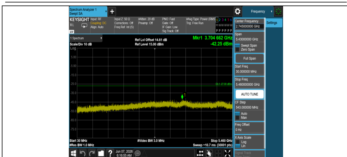
11AC20MIMO-Ant2-5700-30~5460-PASS
