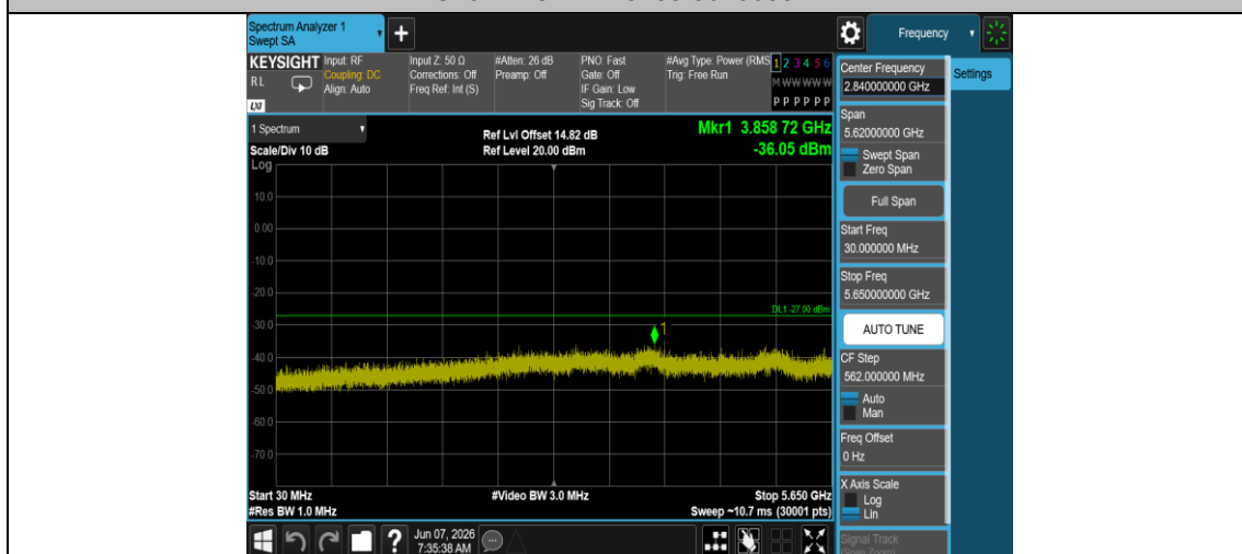
11AC20MIMO-Ant2-5785-30~5650-PASS
