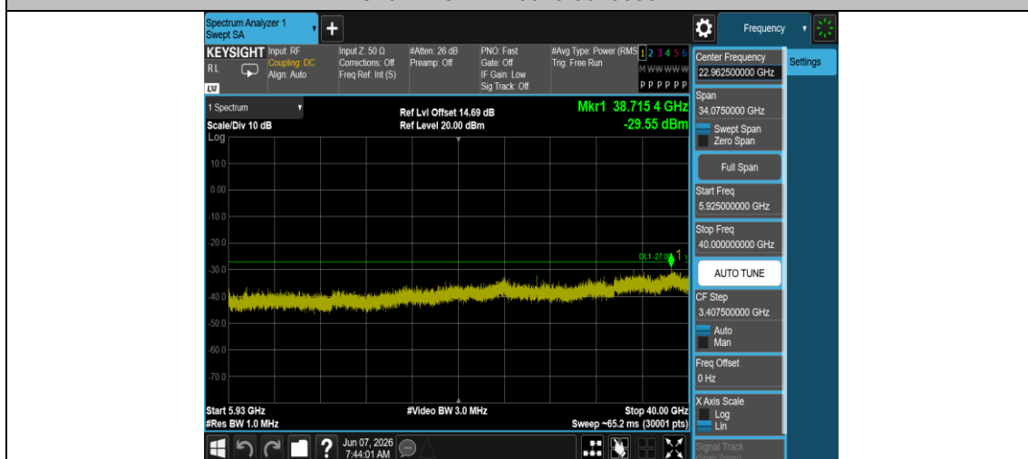
11AC20MIMO-Ant1-5825-5925~40000-PASS
