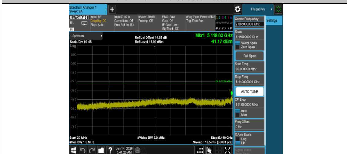
11AC40MIMO-Ant1-5270-30~5140-PASS
