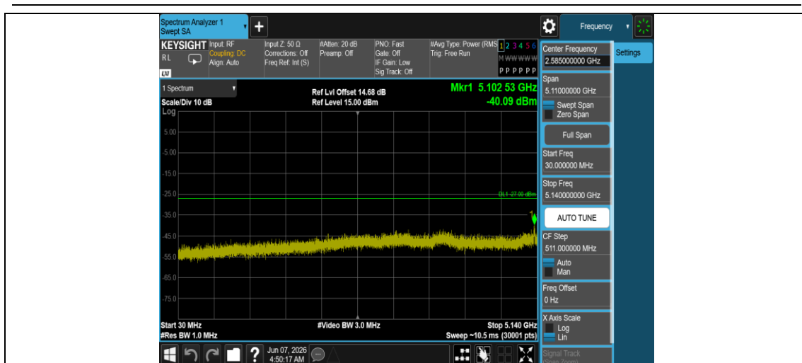
11AC20MIMO-Ant1-5260-30~5140-PASS
