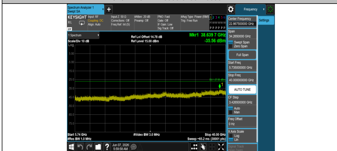
11AC20MIMO-Ant2-5580-5735~40000-PASS
