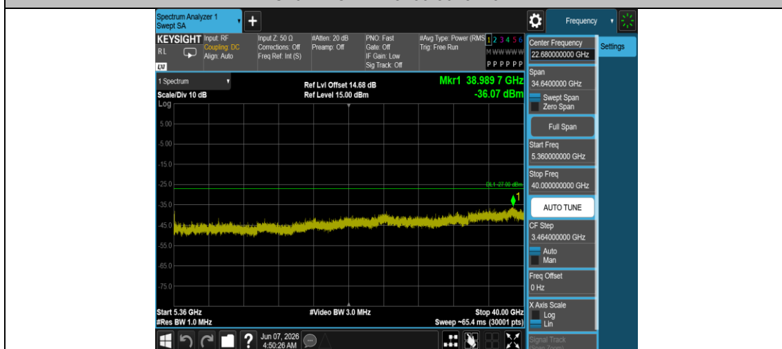
11AC20MIMO-Ant1-5260-5360~40000-PASS
