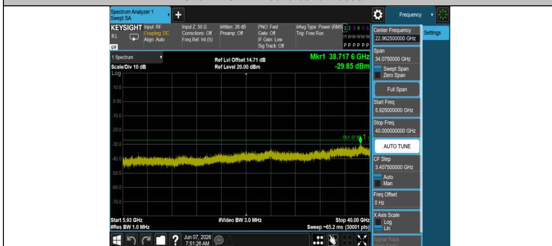
11AC20MIMO-Ant2-5825-5925~40000-PASS
