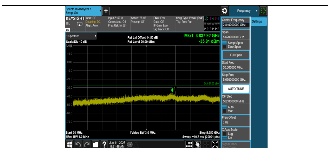
11AX20MIMO-Ant2-5745-30~5650-PASS
