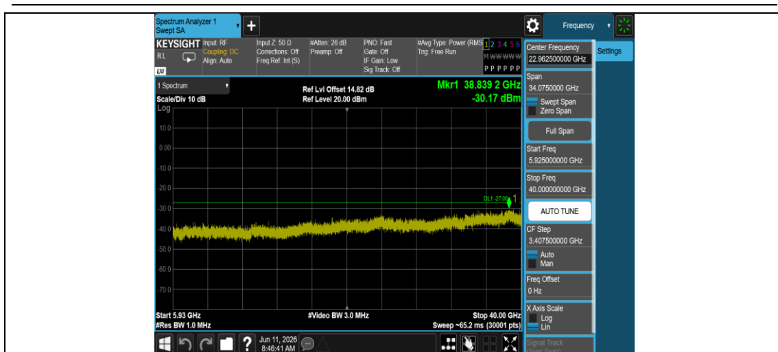
11AX20MIMO-Ant2-5785-5925~40000-PASS
