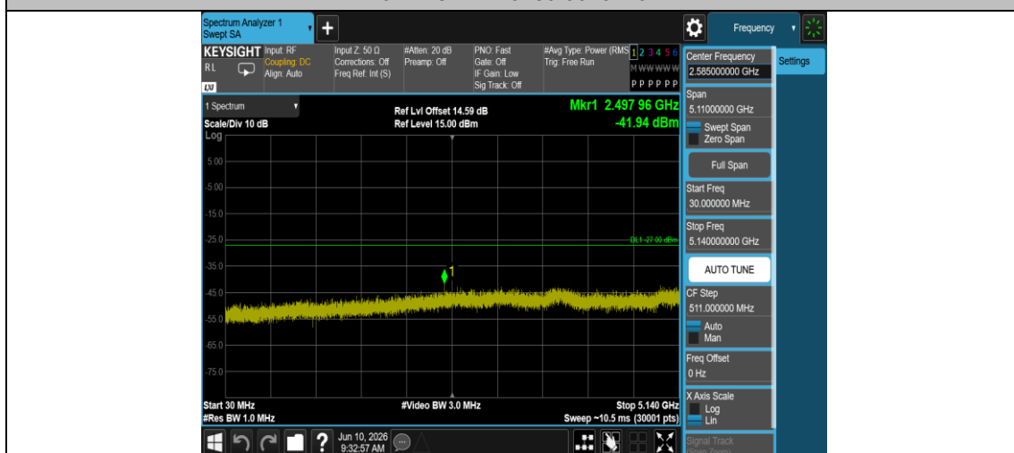
11AX20MIMO-Ant2-5280-30~5140-PASS
