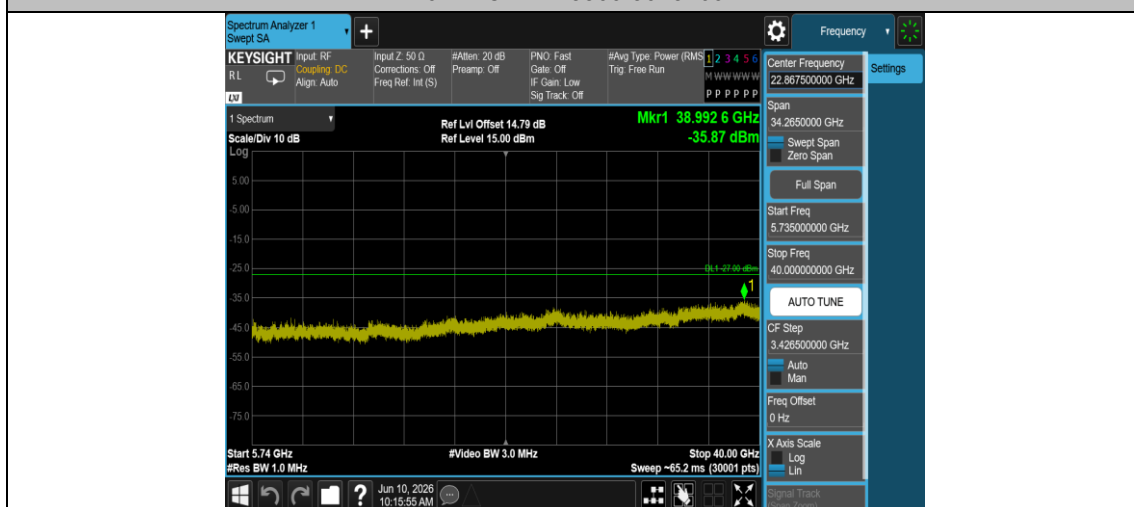
11AX20MIMO-Ant1-5500-5735~40000-PASS
