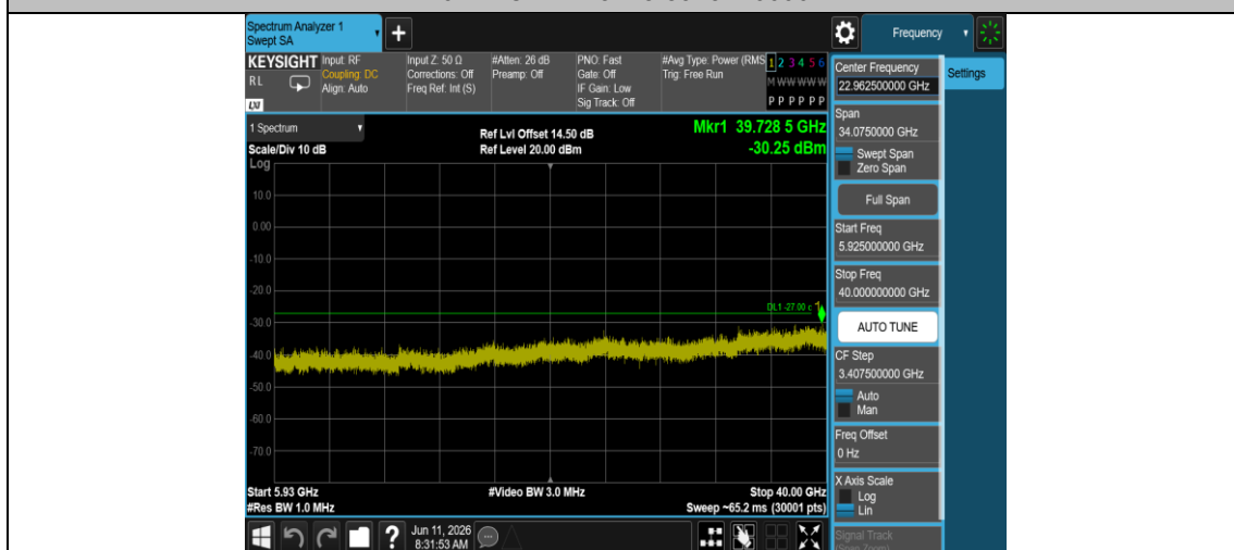
11AX20MIMO-Ant2-5745-5925~40000-PASS
