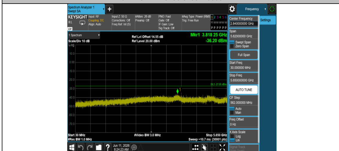
11AX20MIMO-Ant1-5745-30~5650-PASS
