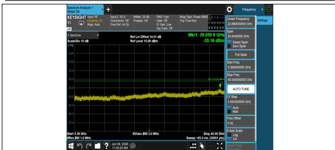
11AX20MIMO-Ant1-5240-5360~40000-PASS
