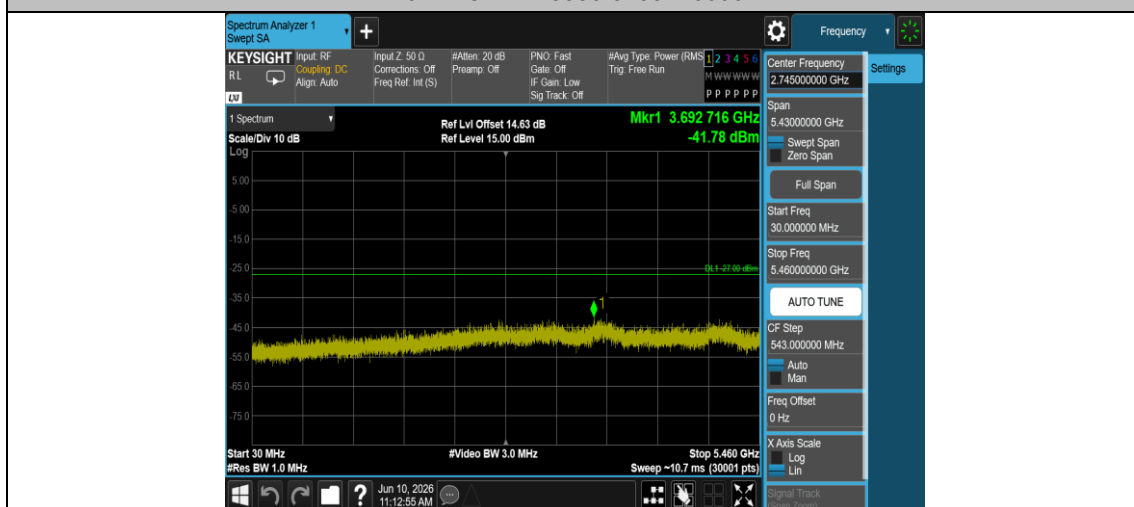
11AX20MIMO-Ant1-5700-30~5460-PASS
