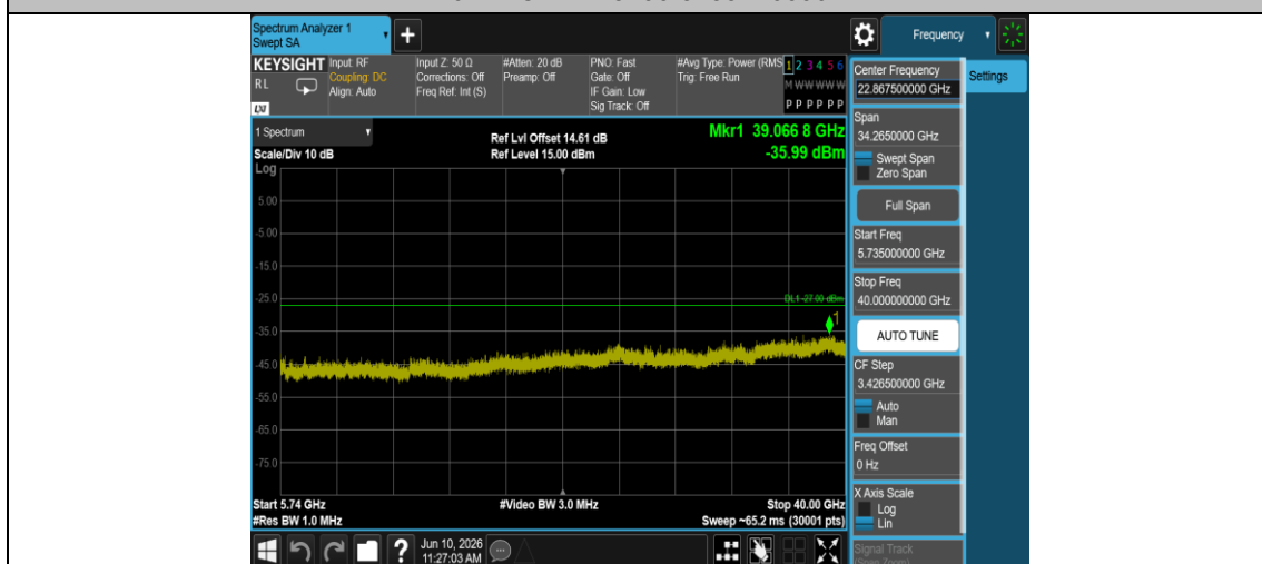
11AX20MIMO-Ant2-5700-5735~40000-PASS
