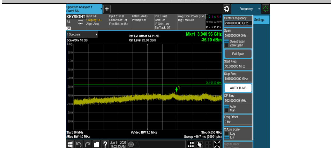
11AX20MIMO-Ant2-5825-30~5650-PASS
