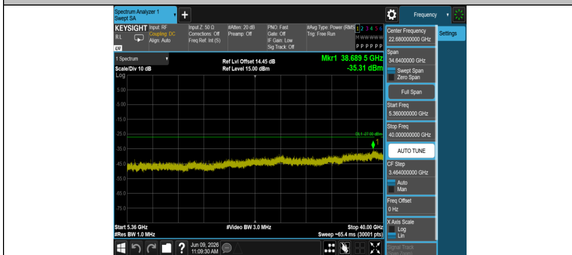
11AX20MIMO-Ant2-5240-5360~40000-PASS
