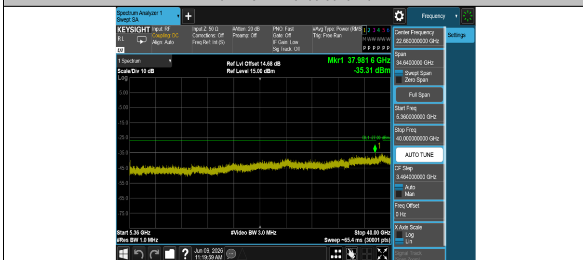
11AX20MIMO-Ant1-5260-5360~40000-PASS
