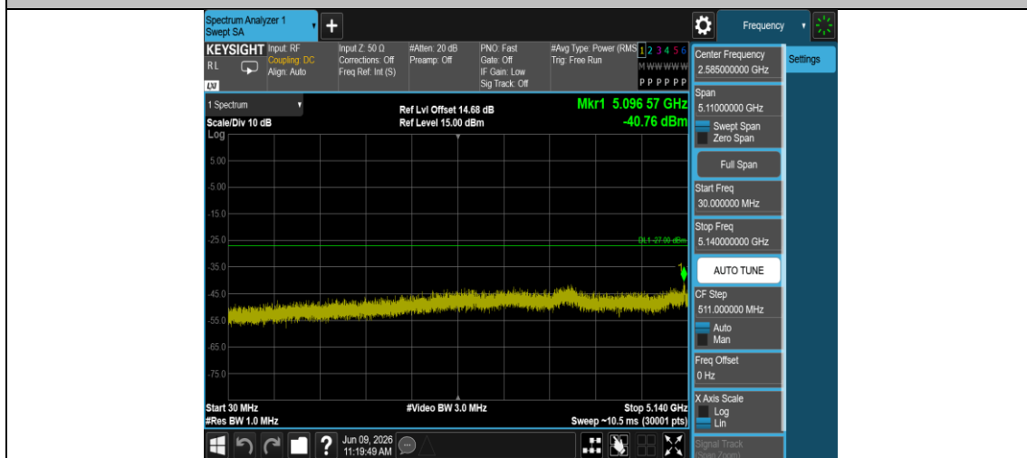
11AX20MIMO-Ant1-5260-30~5140-PASS
