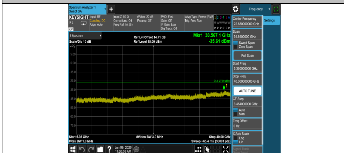
11AX20MIMO-Ant2-5260-5360~40000-PASS
