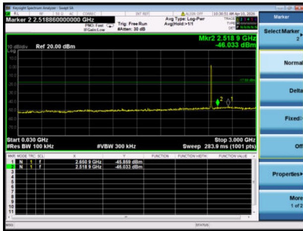
GFSK (BLE 2Mbps) MIDDLE CHANNEL, SPURIOUS 30 MHz ~ 3 GHz
