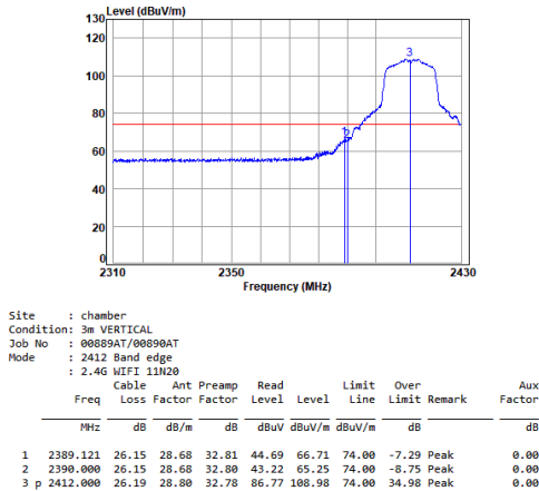
11n_HT(20M)_TX_CH_01_Vertical-Peak
