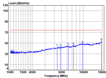
11ax_20M_TX_CH_06_Horizontal-Peak
