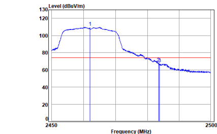
11n_HT(20M)_TX_CH_11_Vertical-Peak
