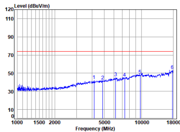
11ax_20M_TX_CH_06_Vertical-Peak
