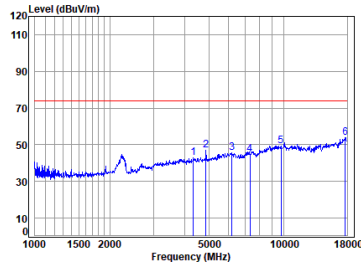
11b_TX_CH_06_Horizontal-Peak
