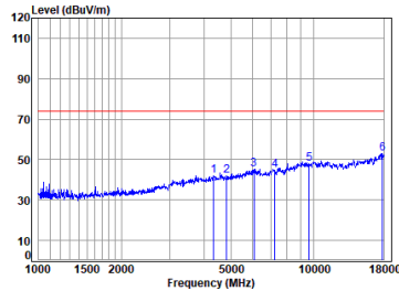
11n_HT(20M)_TX_CH_01_Horizontal-Peak
