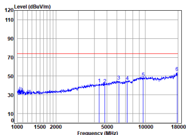
11ax_20M_TX_CH_01_Horizontal-Peak
