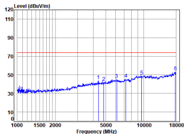
11ax_20M_TX_CH_01_Vertical-Peak
