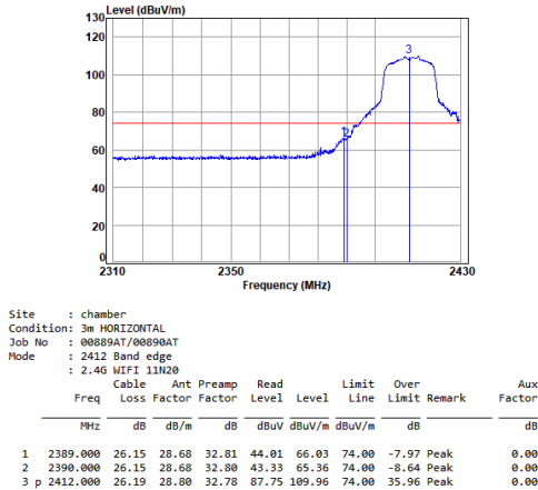
11n_HT(20M)_TX_CH_01_Horizontal-Peak
