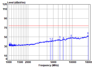
11n_HT(20M)_TX_CH_01_Vertical-Peak
