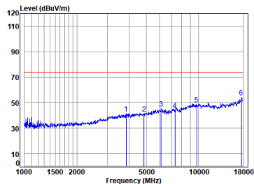
11n_HT(20M)_TX_CH_06_Vertical-Peak
