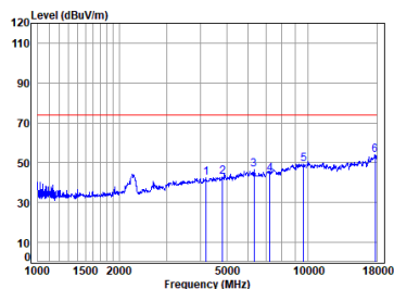
11b_TX_CH_01_Horizontal-Peak
