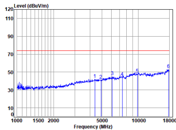
11n_HT(20M)_TX_CH_11_Vertical-Peak
