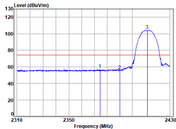
11b_TX_CH_01_Vertical-Peak
