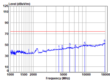
11b_TX_CH_01_Vertical-Peak
