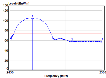
11b_TX_CH_11_Vertical-Peak
