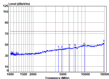
11n_HT(20M)_TX_CH_06_Horizontal-Peak
