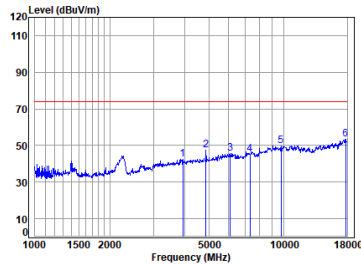
11b_TX_CH_06_Vertical-Peak
