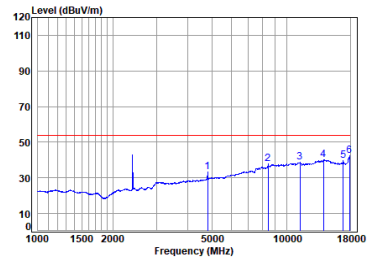
BLE_2M_TX_CH_00_Horizontal-Avg
