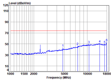
BLE_1M_TX_CH_19_Horizontal-Peak
