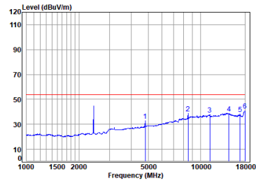
BLE_1M_TX_CH_19_Horizontal-Avg
