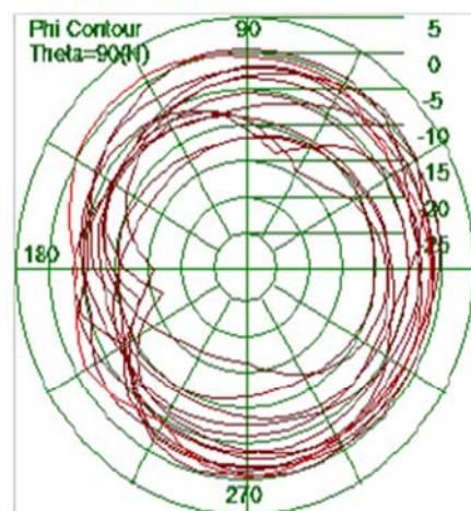
2500 MHz H
