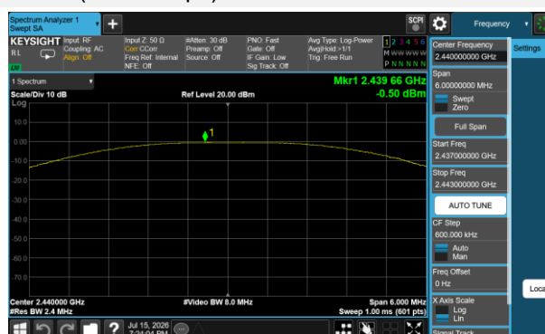
GFSK (BLE 2Mbps) MIDDLE CHANNEL
