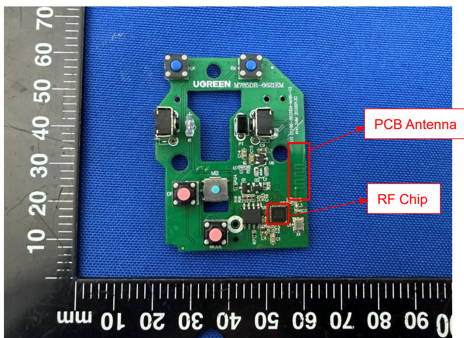
SECONDARY BOARD 2 TOP VIEW
