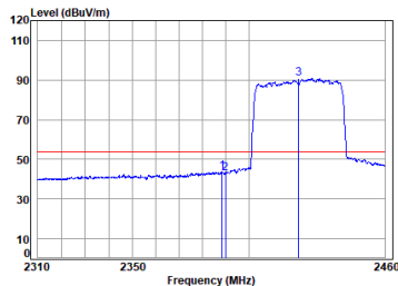
11ax_40M_TX_CH_03_Vertical-Avg
