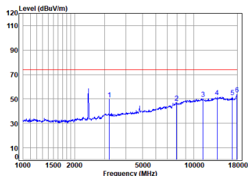
11g_TX_CH_01_Horizontal-Peak
