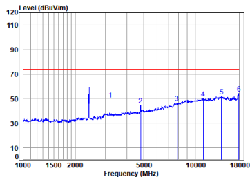
11g_TX_CH_01_Vertical-Peak
