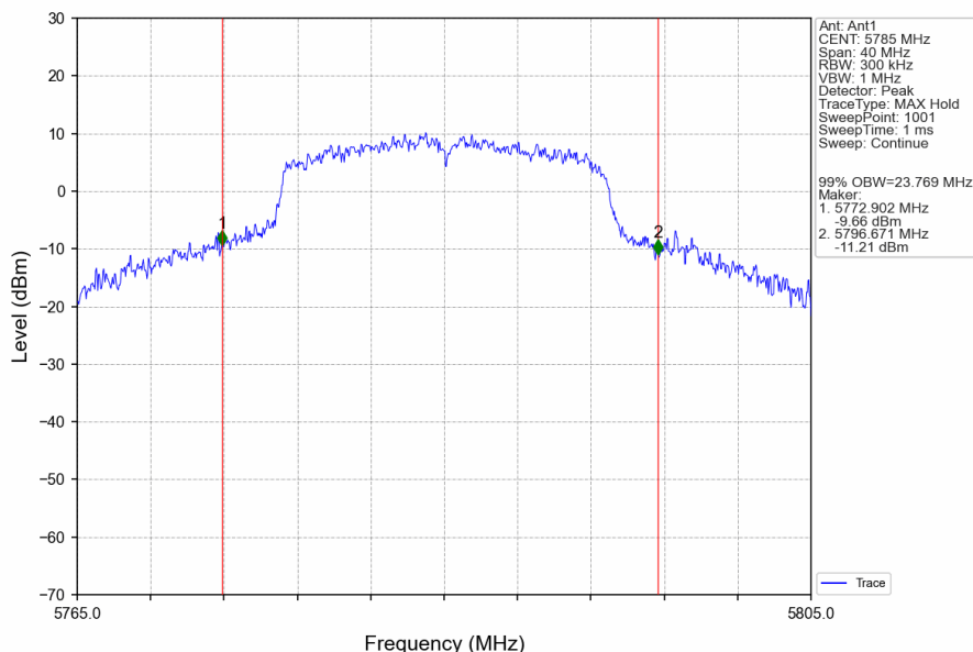
802.11ac(VHT20)_MCH_5785MHz_Ant1_NTNV
