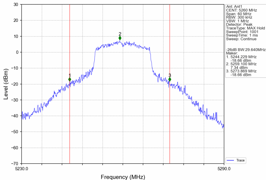
802.11a_LCH_5260MHz_Ant1_NTNV
