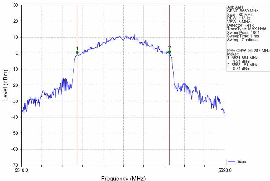
802.11ax(HEW40)_MCH_5550MHz_SU_ / _Ant1_NTNV
